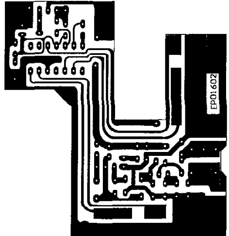
81216 TRANSMITTER PCB SCALE 1:1
