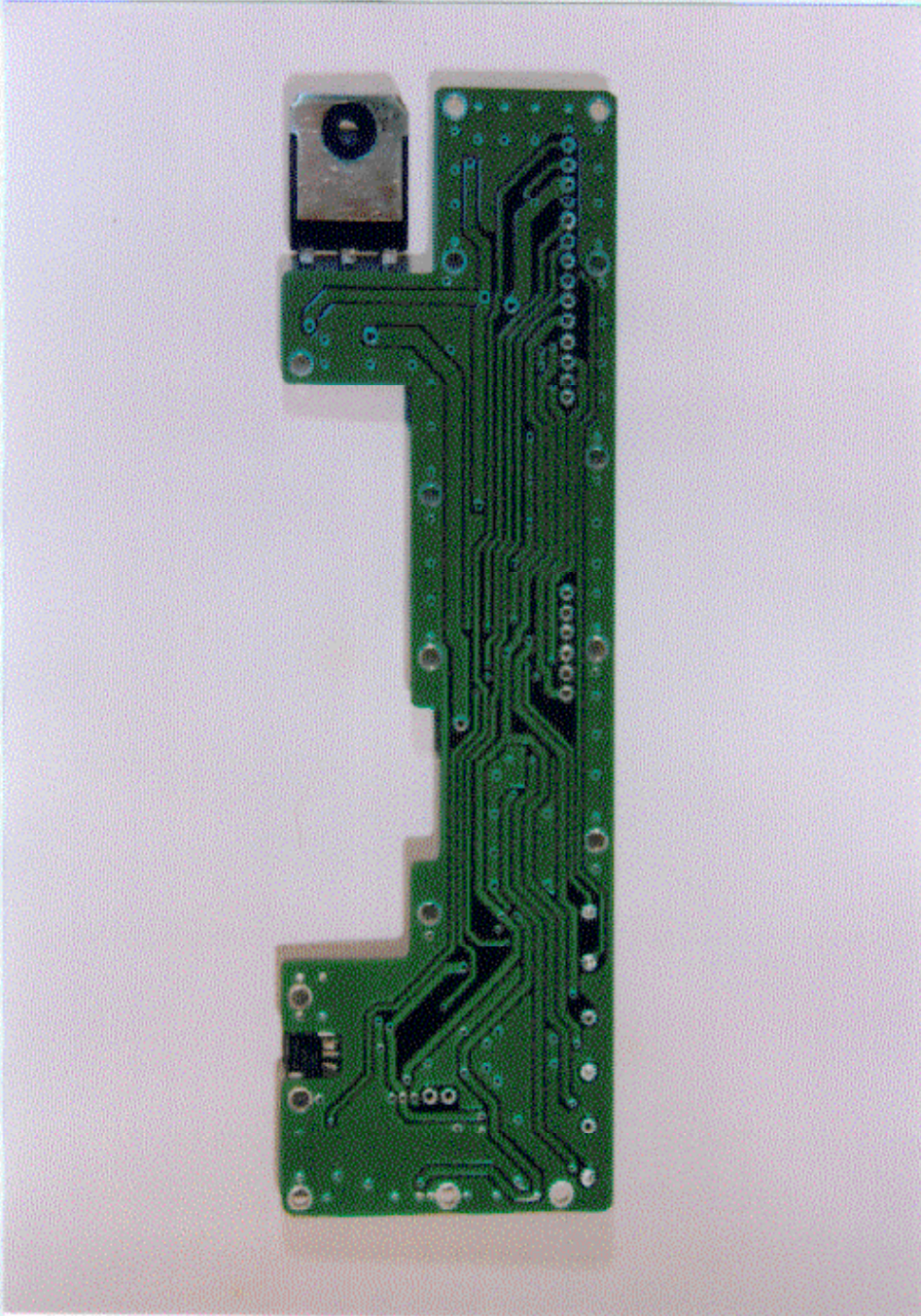
RF board (A3) bottom view
