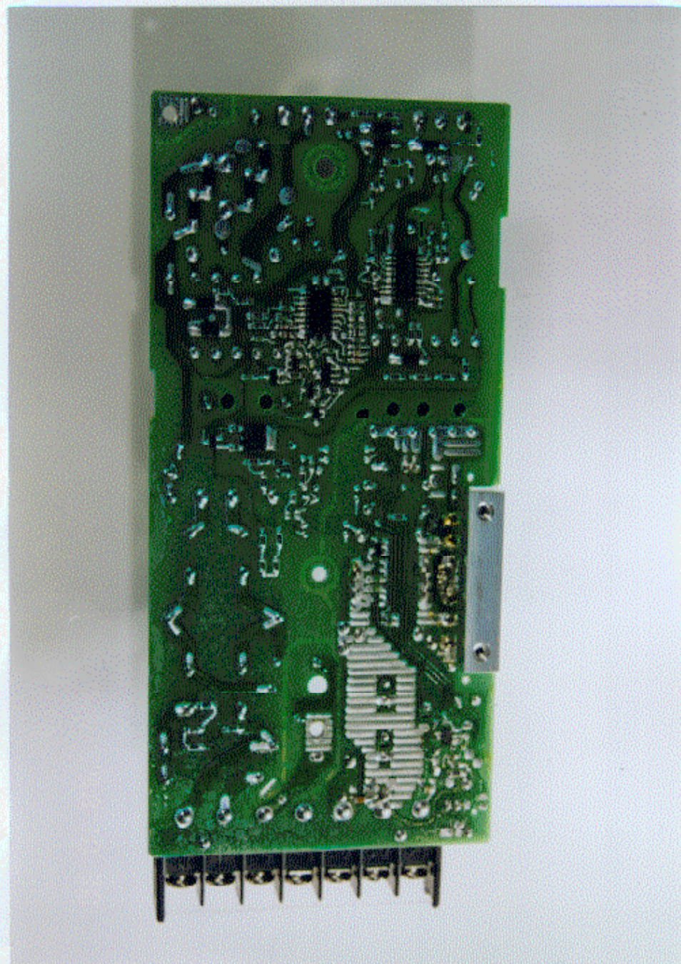
Power Supply Unit (bottom view)
