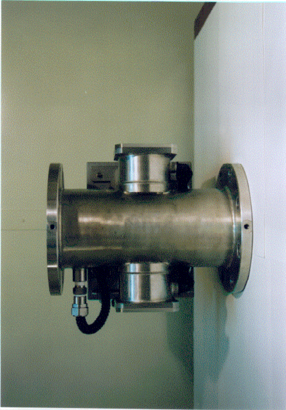
LG 300 Density Meter (bottom side)
