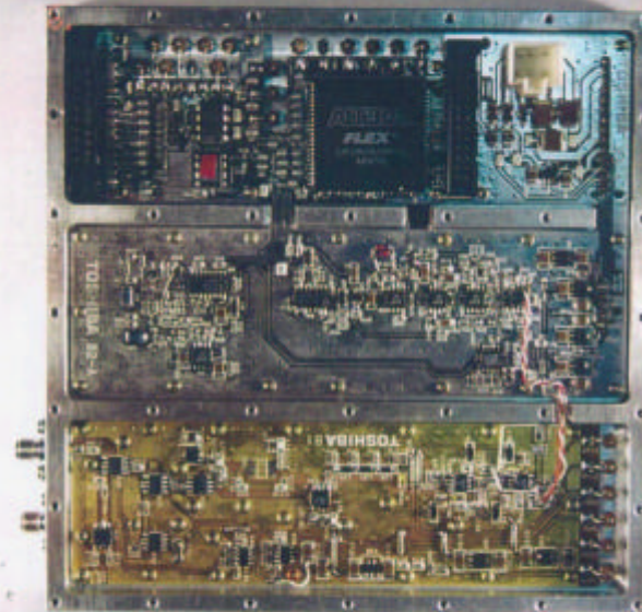
Inside of RF unit (bottom view)
