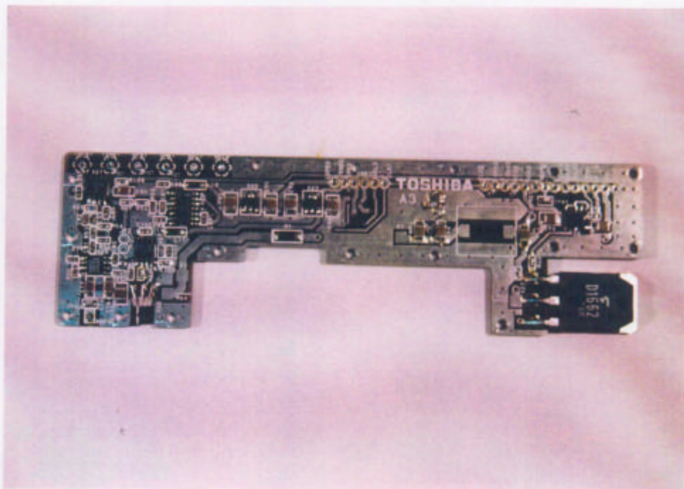
RF board (A3) top view
