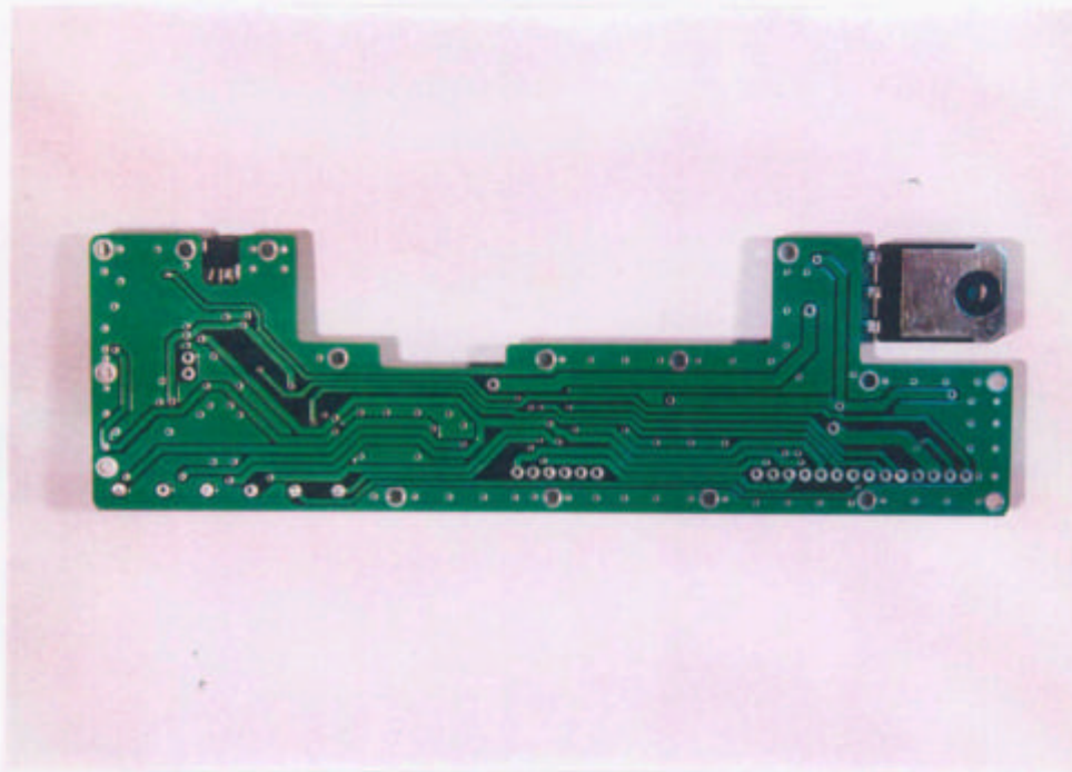
RF board (A3) bottom view
