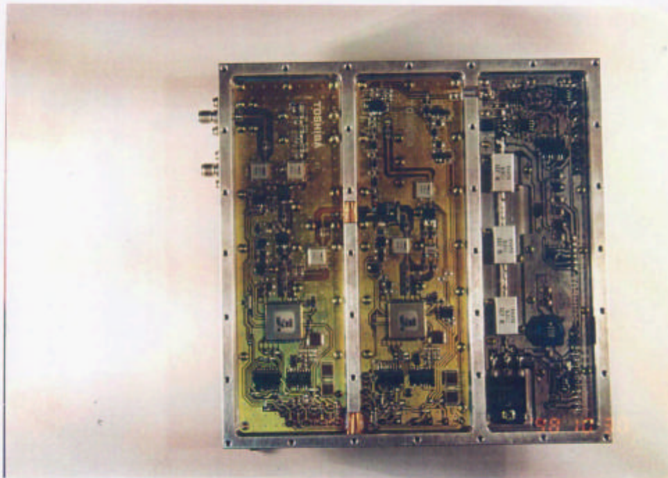
Inside of RF unit (top view)
