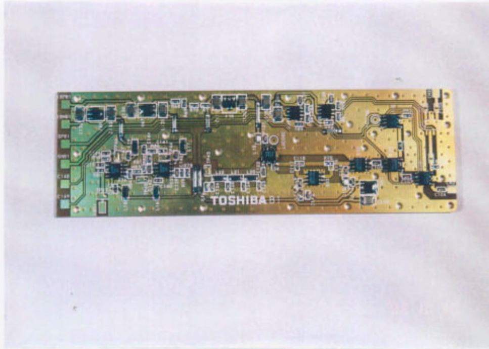
RF board (B1) top view
