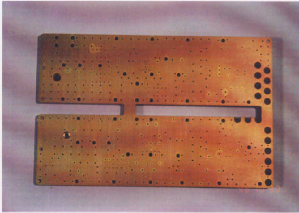
RF board (A1) bottom view
