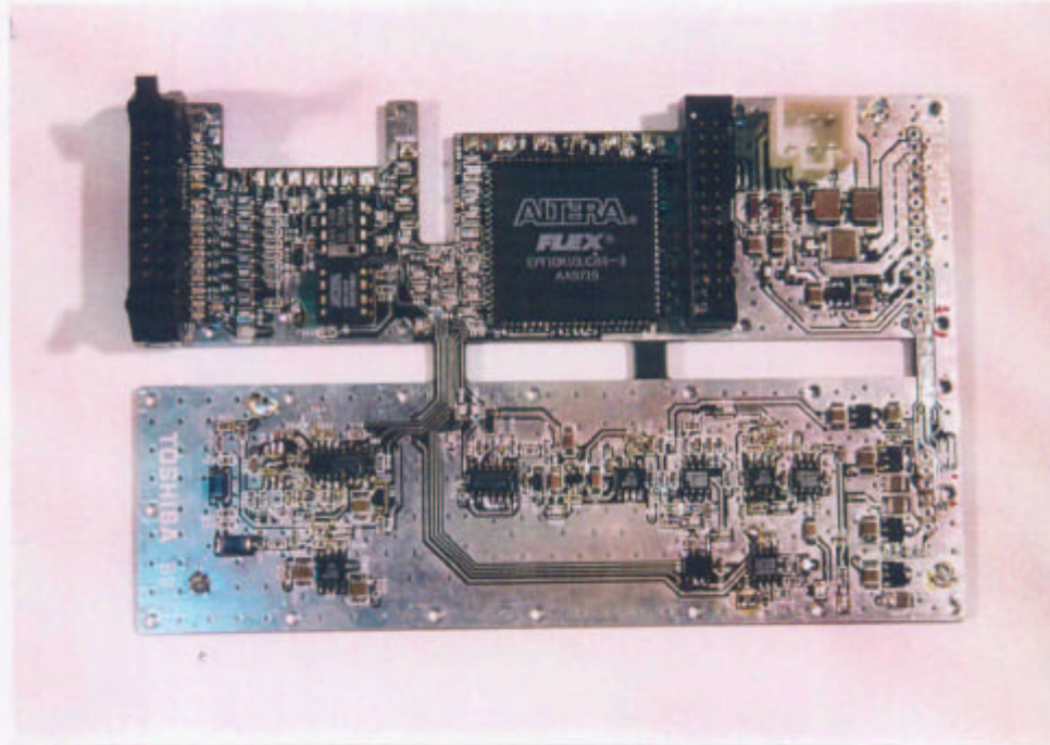
RF board (B2) top view
