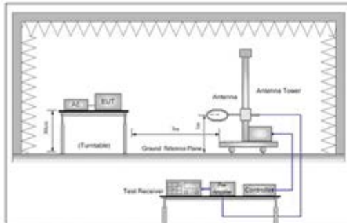
Figure 1. Below 30MHz
