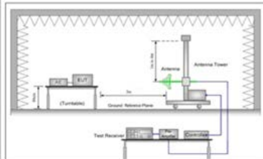
Figure 2. 30MHz to 1GHz.
