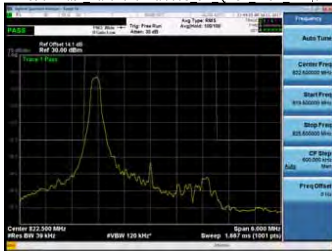
Emission Mask Band26 for Part 90S 3M QPSK HIGH RB1,0
