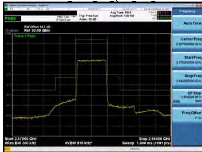
Emission Mask Band 7 15M QPSK LOW RB75,0
