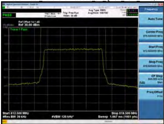
Emission Mask Band26 for Part 90S 3M QPSK LOW RB15,0
