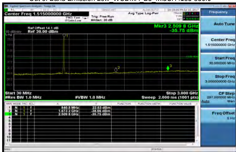
Out of Band Emission Low WCDMA B5 MidCH4183-836.6
