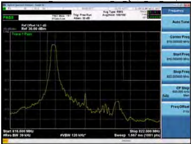
Emission Mask Band26 for Part 90S 3M QPSK MID RB1,0
