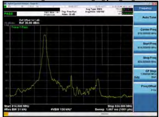
Emission Mask Band26 for Part 90S 5M QPSK MID RB1,0
