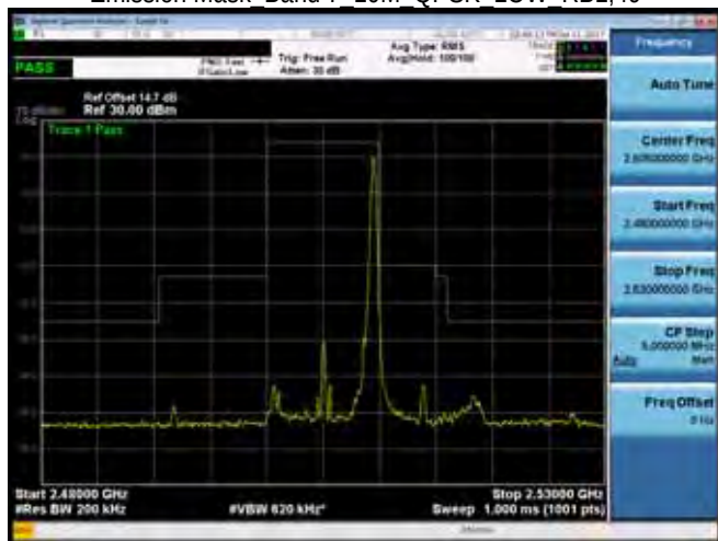
Emission Mask Band 7 10M QPSK LOW RB1,49
