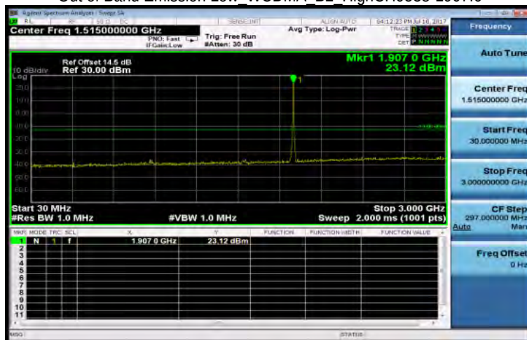
Out of Band Emission Low WCDMA B2 HighCH9538-1907.6
