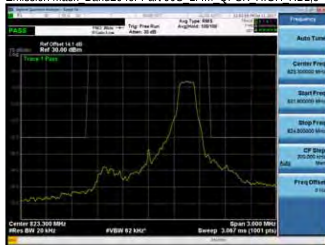
Emission Mask Band26 for Part 90S 1.4M QPSK HIGH RB1,5
