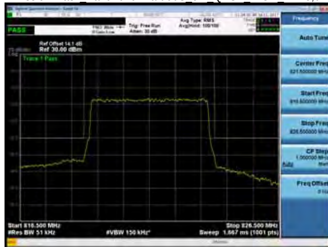
Emission Mask Band26 for Part 90S 5M QPSK HIGH RB25,0
