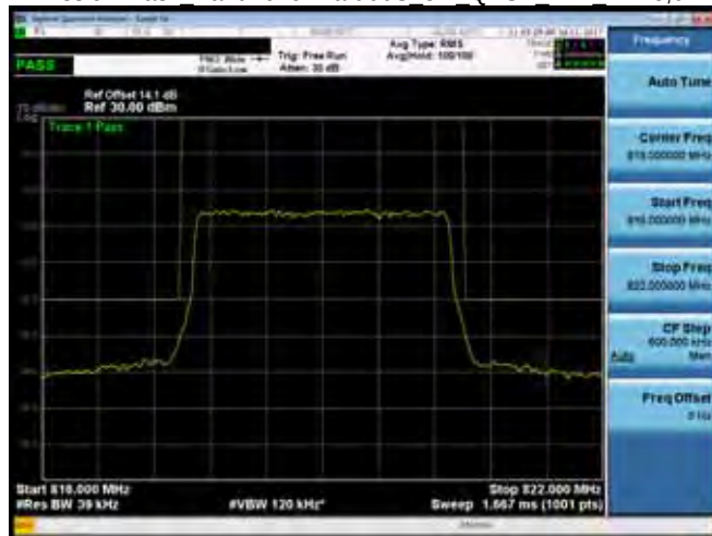
Emission Mask Band26 for Part 90S 3M QPSK MID RB15,0
