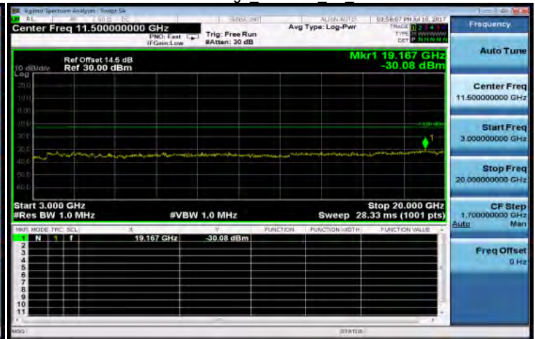
Out of Band Emission High WCDMA B2 HighCH9538-1907.6
