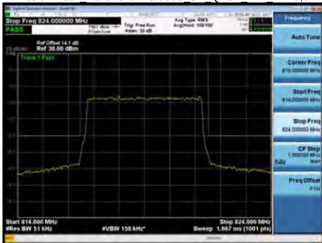
Emission Mask Band26 for Part 90S 5M QPSK MID RB25,0
