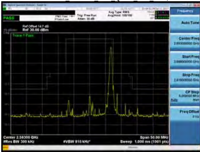
Emission Mask Band 41 15M QPSK MID RB75,0
