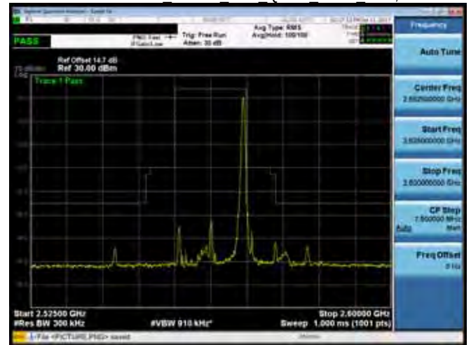
Emission Mask Band 7 15M QPSK HIGH RB75,0
