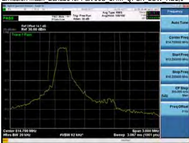
Emission Mask Band26 for Part 90S 1.4M QPSK LOW RB1,0
