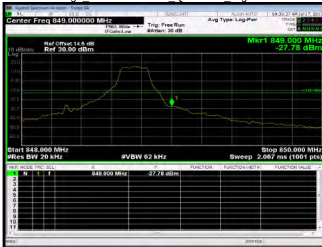
Band Edge_Band26 1.4MHz_QPSK 1 5_High267033-848.3
