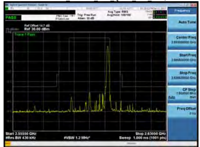
Emission Mask Band 41 20M QPSK MID RB1,99
