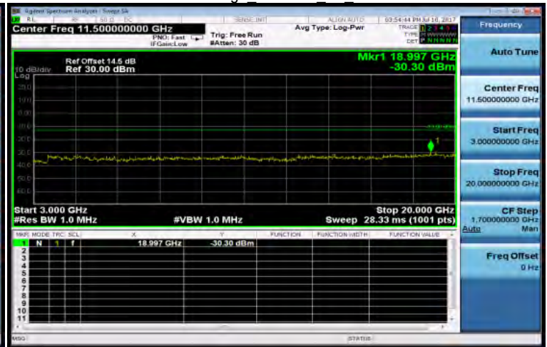
Out of Band Emission High WCDMA B2 LowCH9262-1852.4
