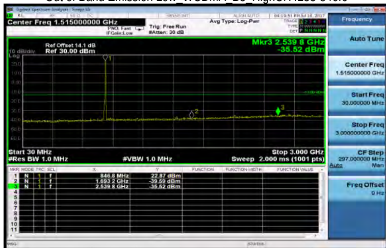
Out of Band Emission Low WCDMA B5 HighCH4233-846.6
