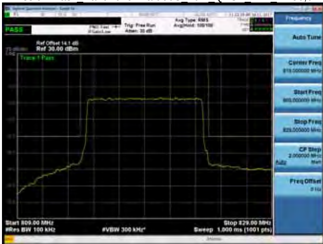
Emission Mask Band26 for Part 90S 10M QPSK MID RB50,0
