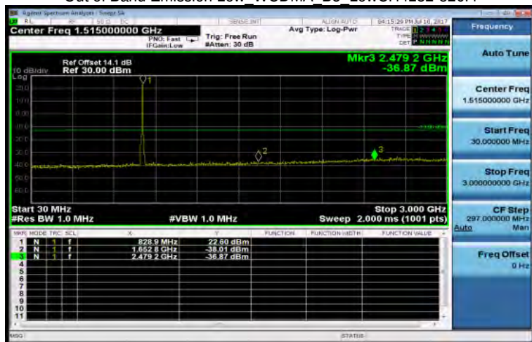
Out of Band Emission Low WCDMA B5 LowCH4132-826.4
