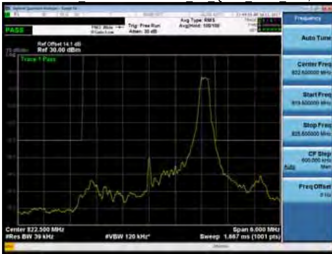
Emission Mask Band26 for Part 90S 3M QPSK HIGH RB15,0
