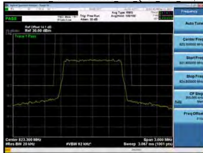
Emission Mask Band26 for Part 90S 1.4M QPSK HIGH RB6,0
