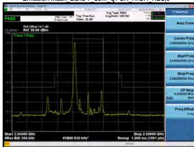
Emission Mask Band 7 10M QPSK HIGH RB1,0
