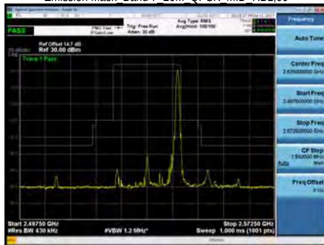
Emission Mask Band 7 20M QPSK MID RB1,99
