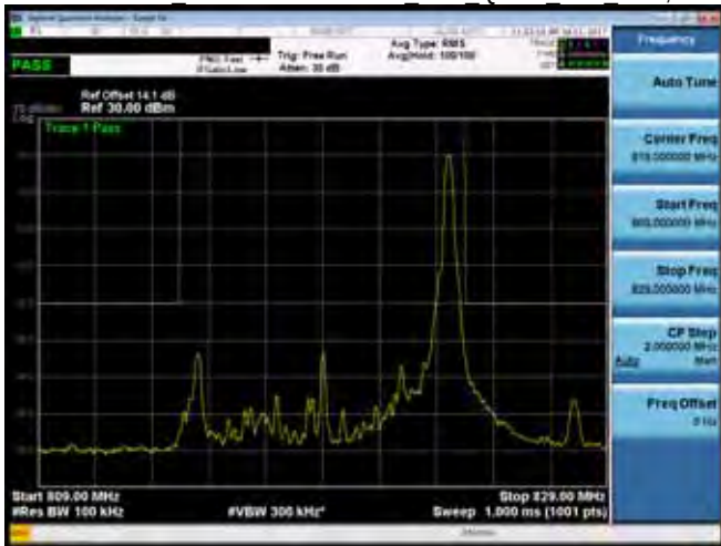
Emission Mask Band26 for Part 90S 10M QPSK MID RB1,49
