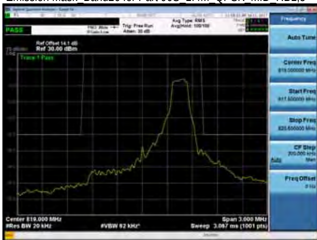
Emission Mask Band26 for Part 90S 1.4M QPSK MID RB1,5
