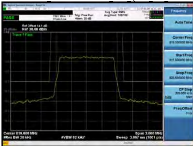
Emission Mask Band26 for Part 90S 1.4M QPSK MID RB6,0
