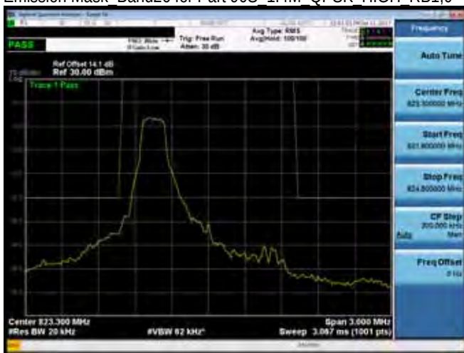
Emission Mask Band26 for Part 90S 1.4M QPSK HIGH RB1,0
