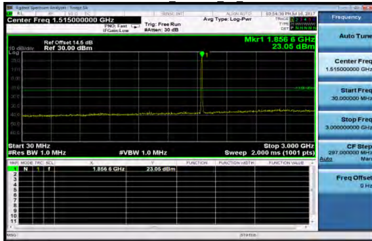
Out of Band Emission Low WCDMA B2 LowCH9262-1852.4
