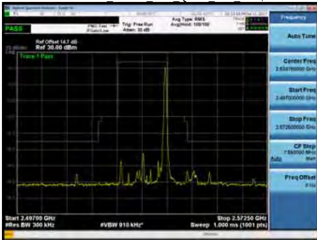
Emission Mask Band 7 15M QPSK MID RB1,74
