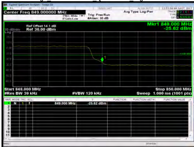
Band Edge Band26 3MHz QPSK 15 0 High CH27025-847.5
