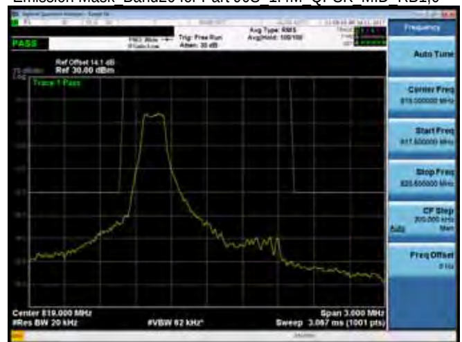
Emission Mask Band26 for Part 90S 1.4M QPSK MID RB1,0
