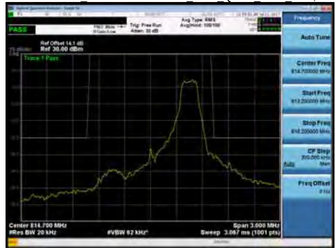
Emission Mask Band26 for Part 90S 1.4M QPSK LOW RB1,5
