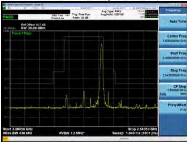
Emission Mask Band 41 20M QPSK LOW RB1,99
