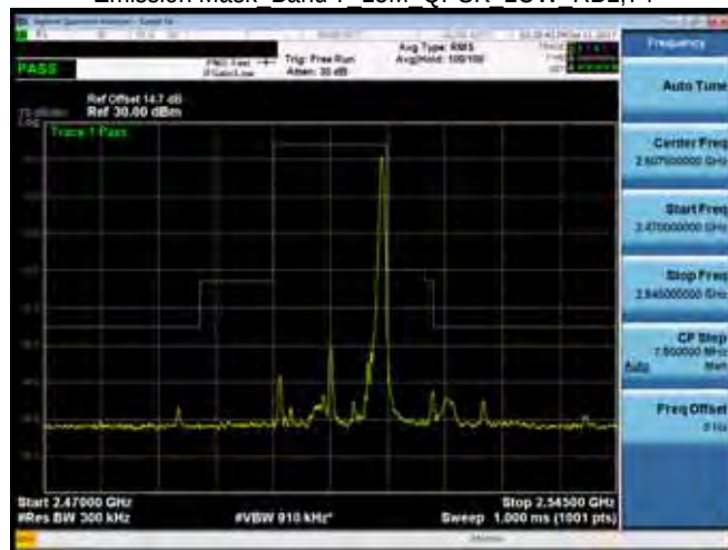
Emission Mask Band 7 15M QPSK LOW RB1,74
