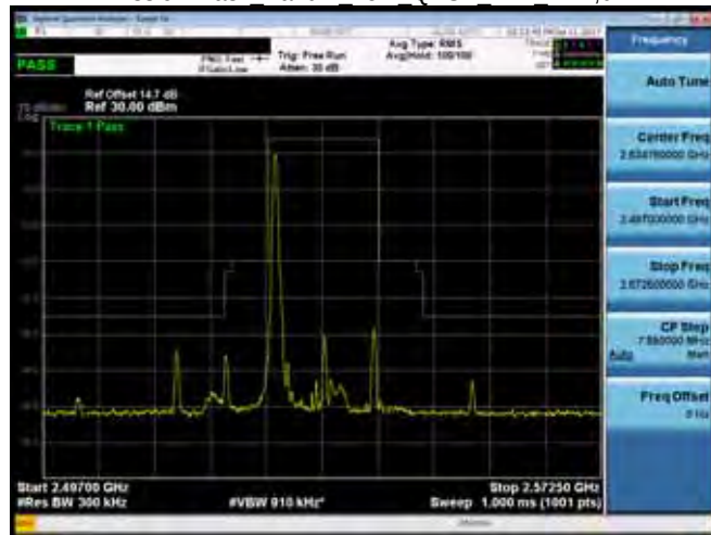
Emission Mask Band 7 15M QPSK MID RB1,0
