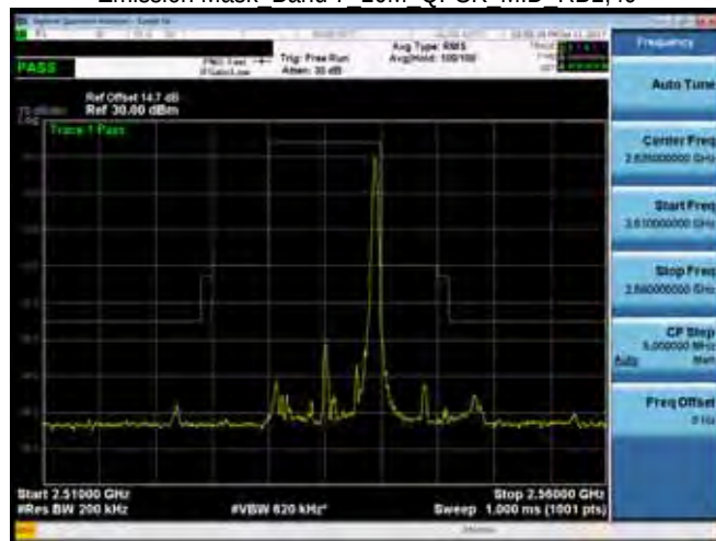
Emission Mask Band 7 10M QPSK MID RB1,49
