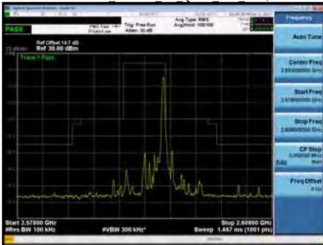
Emission Mask Band 41 5M QPSK MID RB1,24
