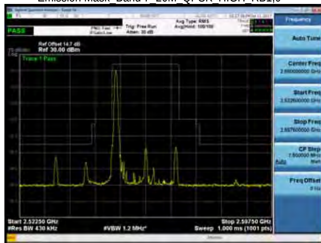
Emission Mask Band 7 20M QPSK HIGH RB1,0
