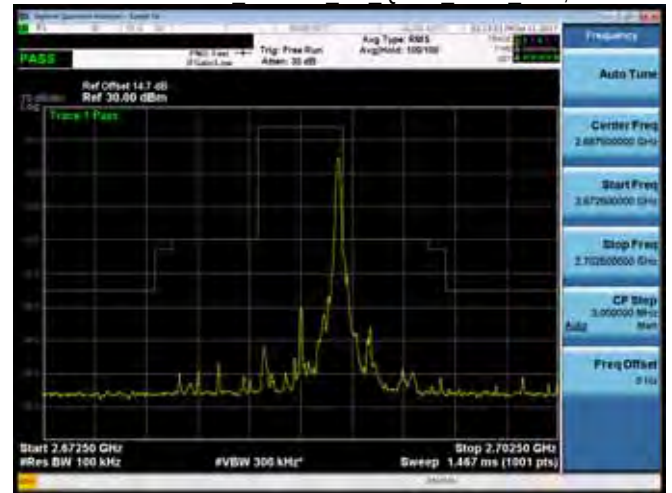
Emission Mask Band 41 5M QPSK HIGH RB1,24
