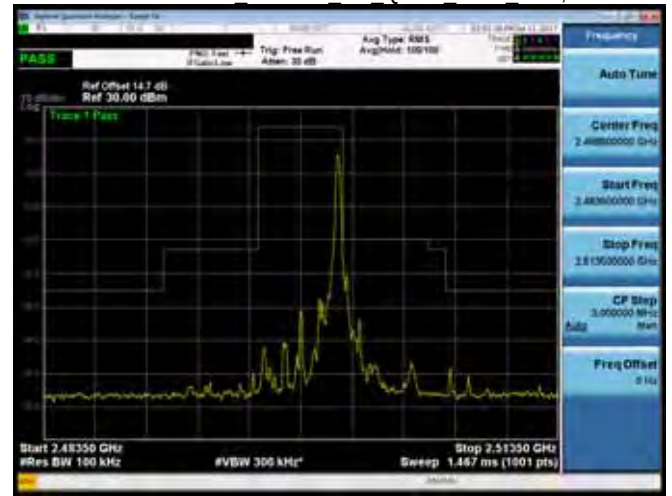
Emission Mask Band 41 5M QPSK LOW RB25,0
