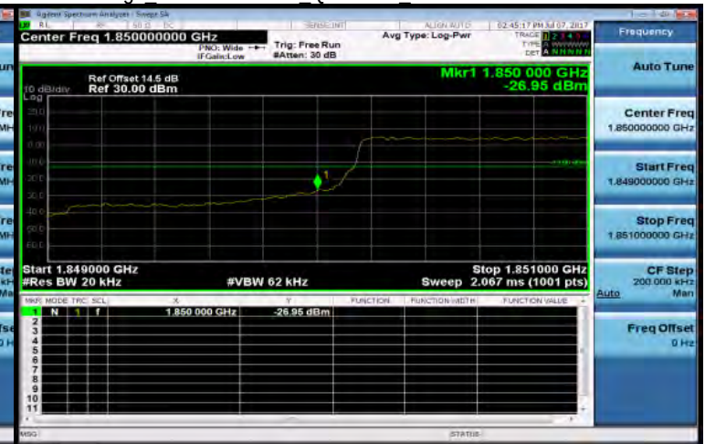
Band Edge_Band25 1.4MHz_QPSK 6 0_LowCH26047-1850.7
