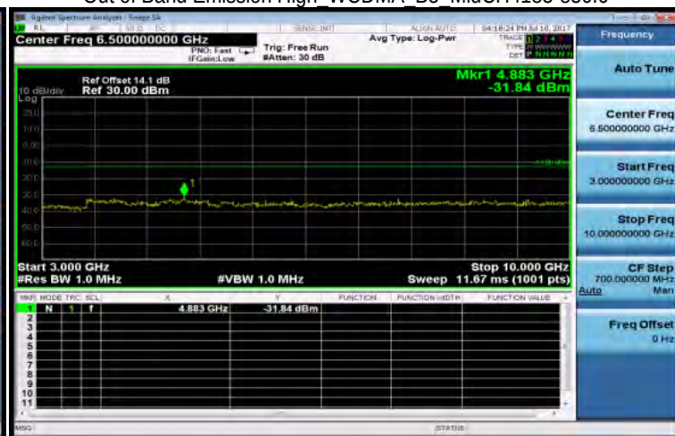
Out of Band Emission High WCDMA B5 MidCH4183-836.6
