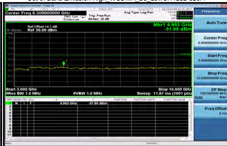
Out of Band Emission High WCDMA B5 LowCH4132-826.4
