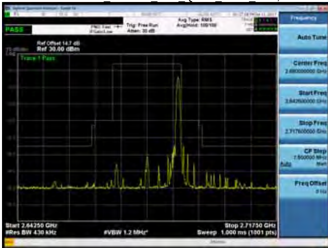
Emission Mask Band 41 20M QPSK HIGH RB1,99
