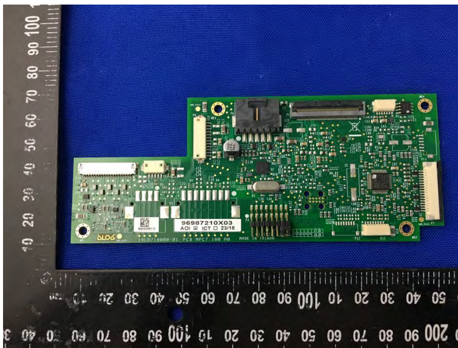
MAIN BOARD 3 TOP VIEW (DLT-V7212P+)
