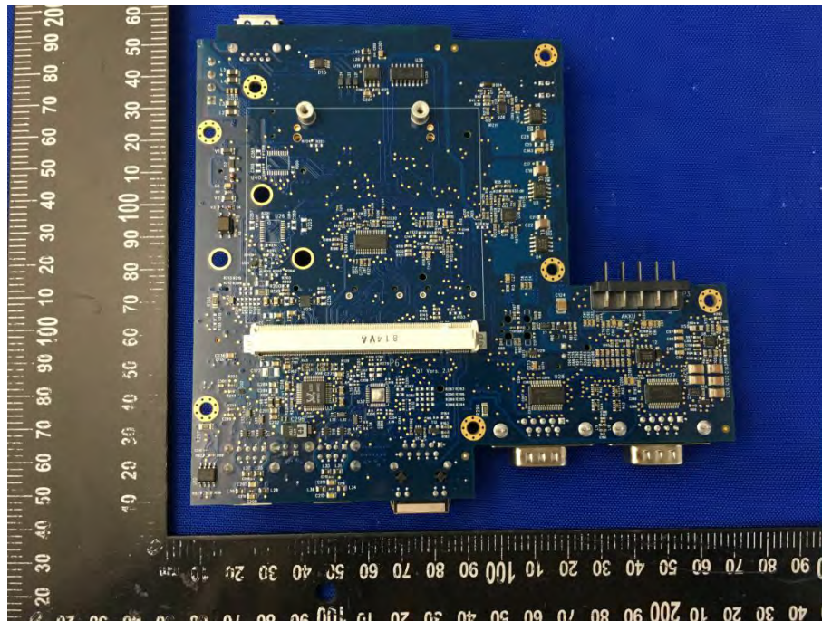
MAIN BOARD 7 REAR VIEW (DLT-V7212P+)
