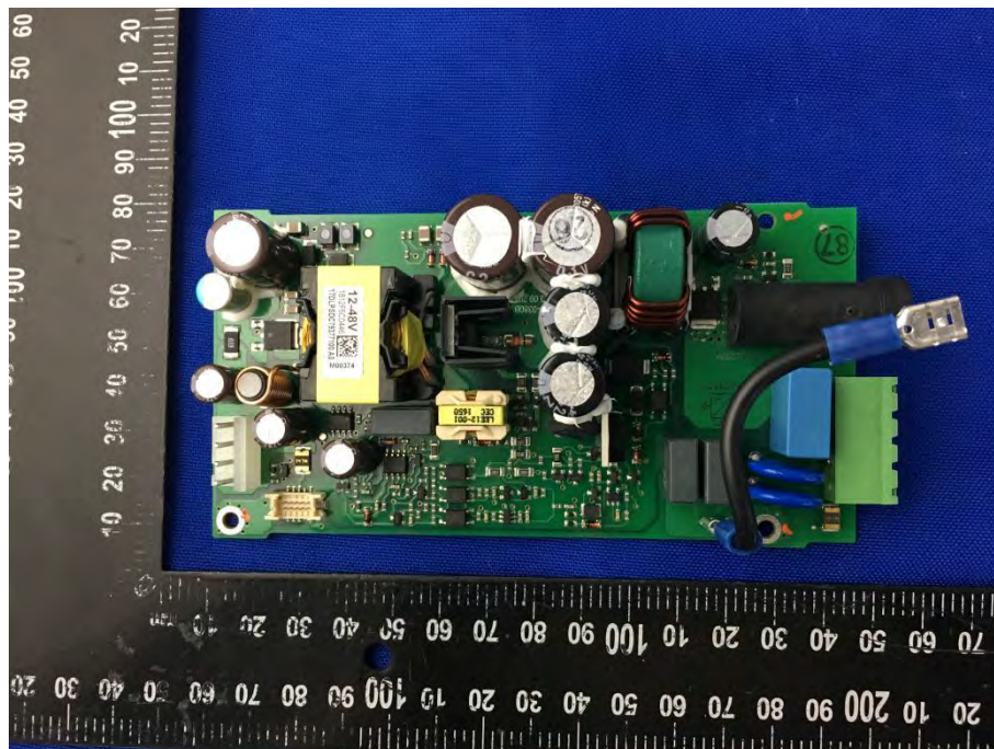
MAIN BOARD 1 TOP VIEW (DLT-V7212P+)
