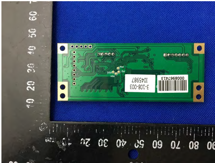
MAIN BOARD 2 REAR VIEW (DLT-V7212P+)
