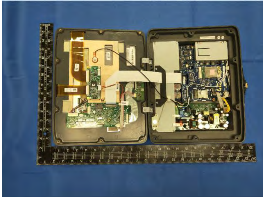
EUT UNCOVER VIEW (DLT-V7212P+)
