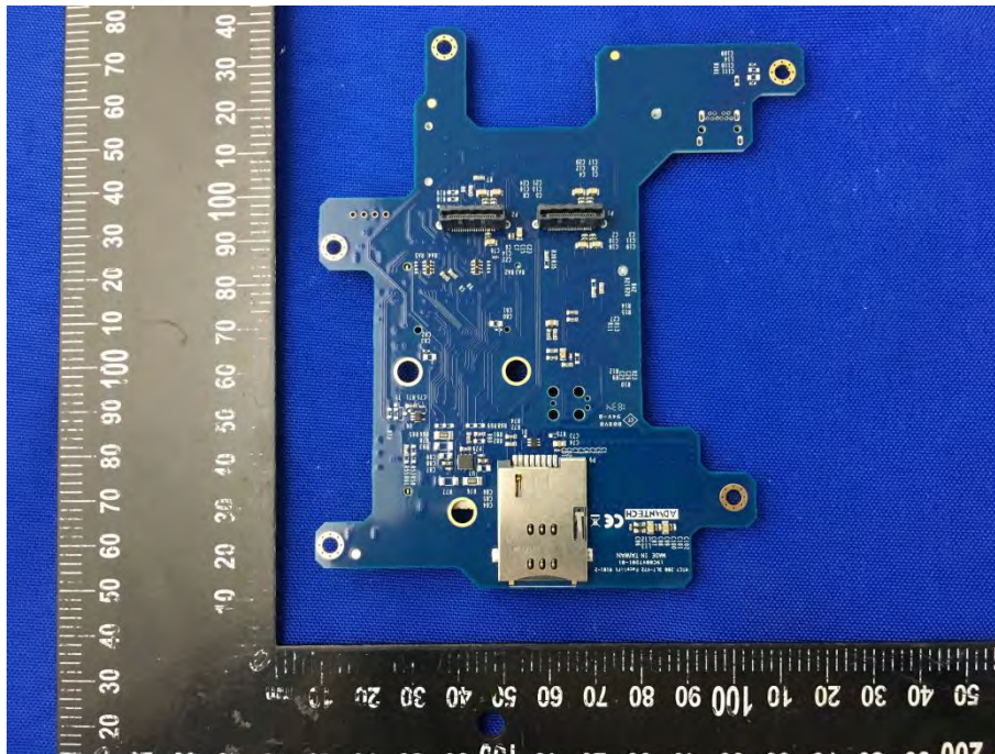
MAIN BOARD 5 REAR VIEW (DLT-V7212P+)
