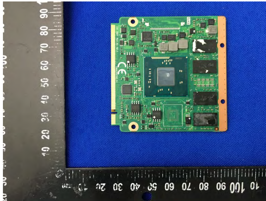
MAIN BOARD 7 TOP VIEW (DLT-V7210P)
