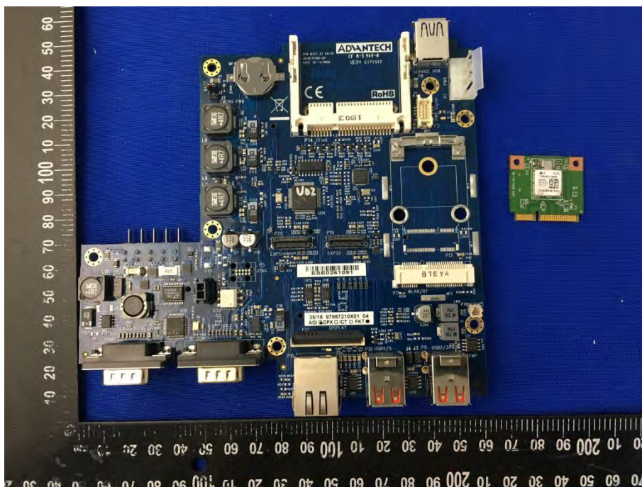
EUT UNCOVER VIEW (DLT-V7210P)
