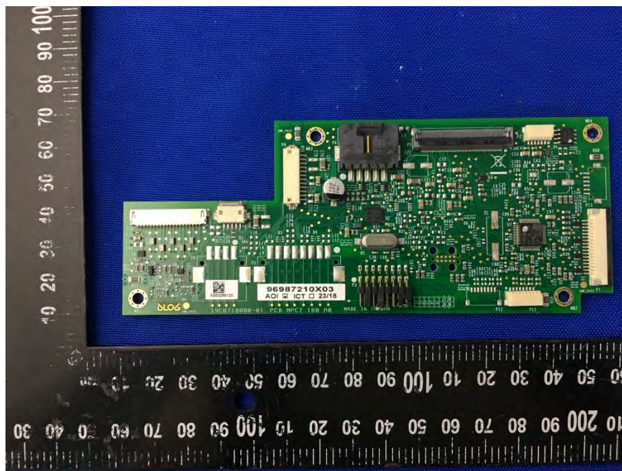
MAIN BOARD 3 TOP VIEW (DLT-V7210P)
