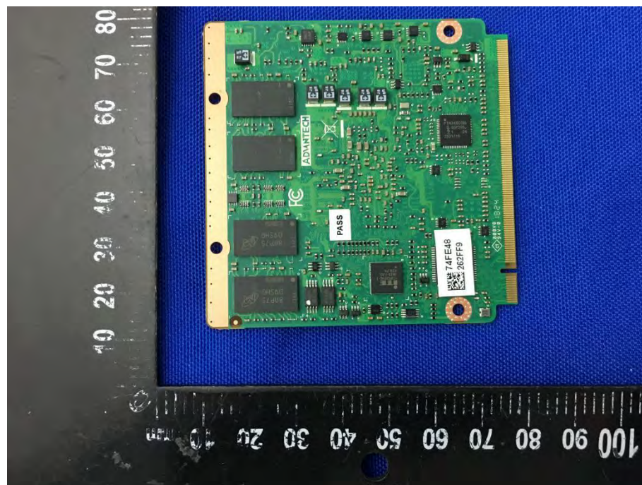
MAIN BOARD 7 REAR VIEW (DLT-V7210P)
