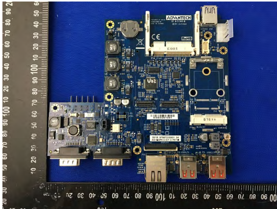
MAIN BOARD 6 TOP VIEW (DLT-V7210P)
