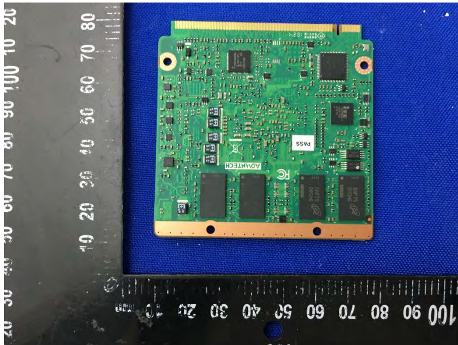
MAIN BOARD 8 REAR VIEW (DLT-V7212P+)
