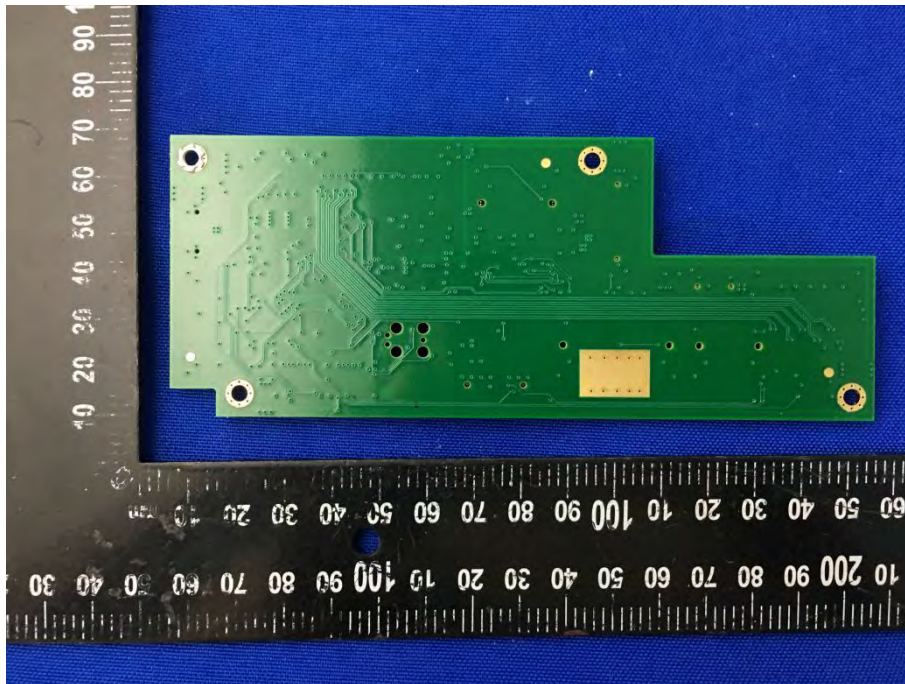
MAIN BOARD 3 REAR VIEW (DLT-V7210P)
