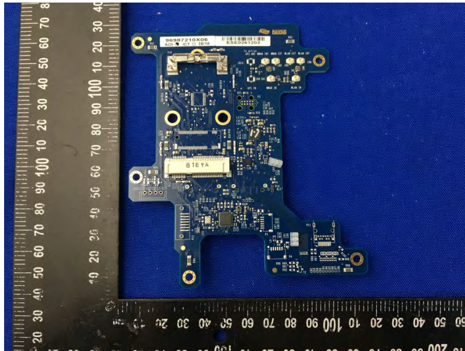
MAIN BOARD 4 TOP VIEW (DLT-V7210P)
