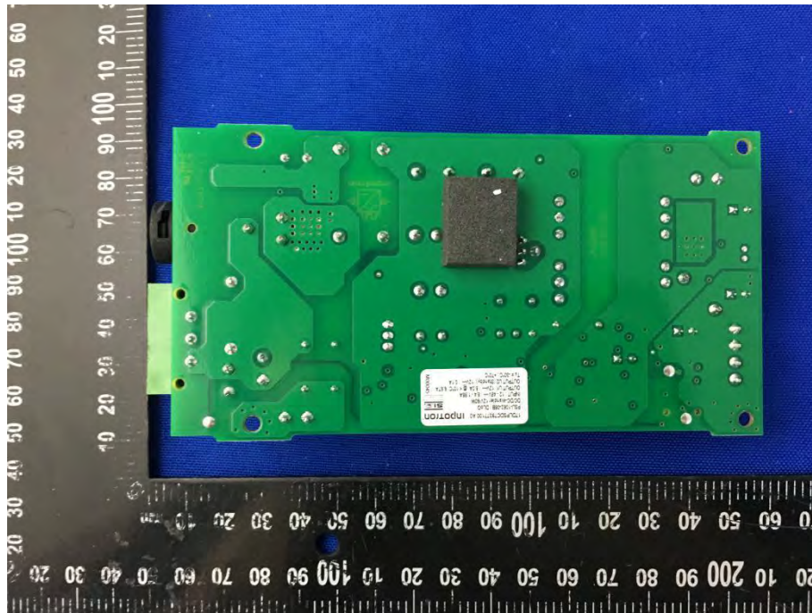
MAIN BOARD 1 REAR VIEW (DLT-V7210P)
