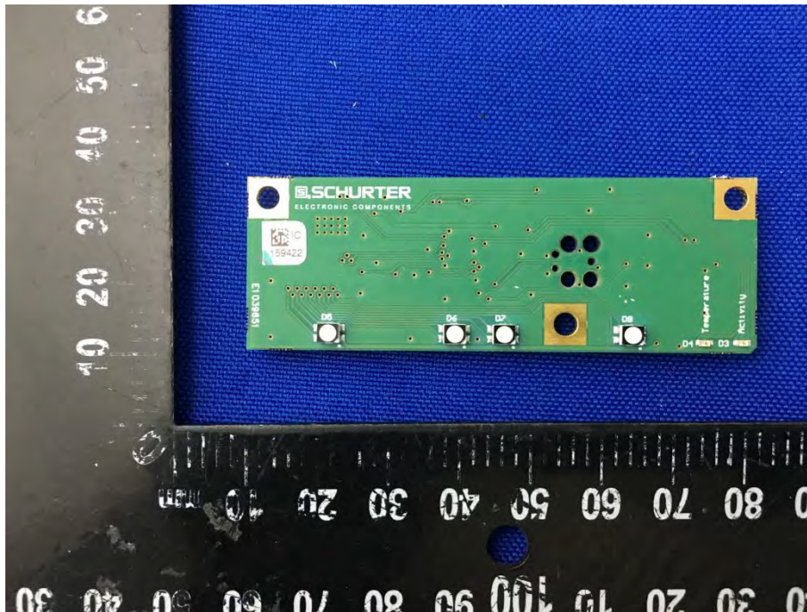
MAIN BOARD 4 REAR VIEW (DLT-V7212P+)
