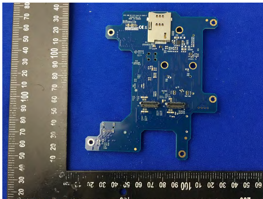
MAIN BOARD 4 REAR VIEW (DLT-V7210P)
