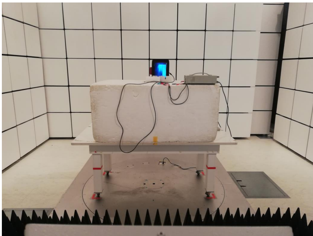
Radiated emissions test photos Above 1 GHz Antenna: Integrated Plane: Y
