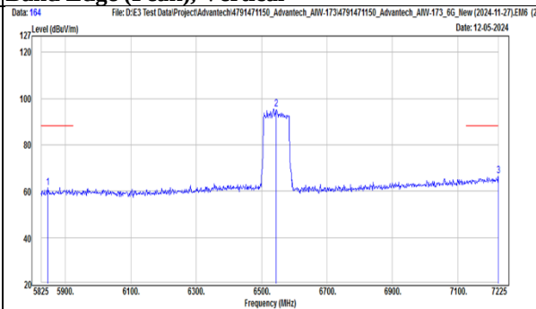
TX, 802.11be(EHT80) (Ch 119) Band Edge (Peak), Vertical
