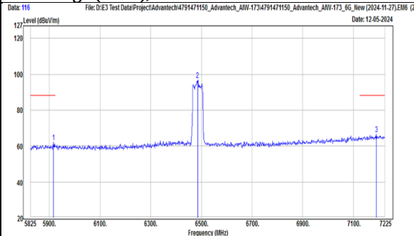
TX, 802.11be(EHT40) (Ch 107) Band Edge (Peak), Vertical
