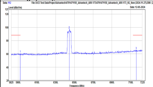
TX, 802.11be(EHT40) (Ch 99) Band Edge (Peak), Vertical
