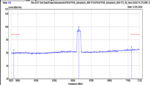
TX, 802.11be(EHT40) (Ch 123) Band Edge (Peak), Vertical
