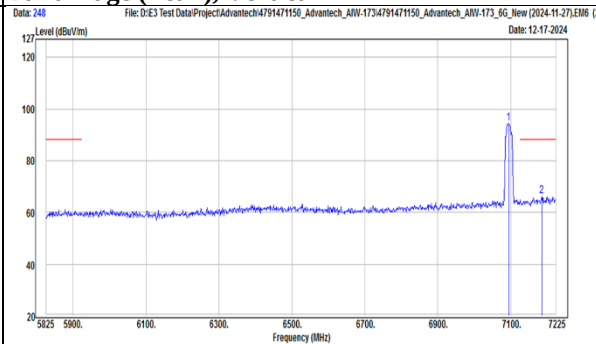
TX, 802.11be(EHT20) (Ch 229) Band Edge (Peak), Vertical
