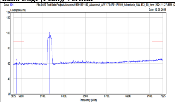
TX, 802.11be(EHT40) (Ch 43) Band Edge (Peak), Vertical
