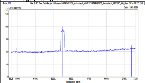
TX, 802.11be(EHT40) (Ch 91) Band Edge (Peak), Vertical
