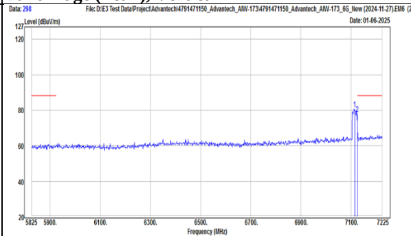
TX, 802.11be(EHT20) (Ch 233) Band Edge (Peak), Vertical
