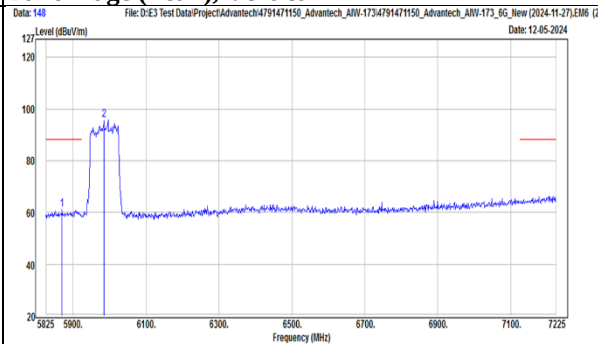
TX, 802.11be(EHT80) (Ch 7) Band Edge (Peak), Vertical
