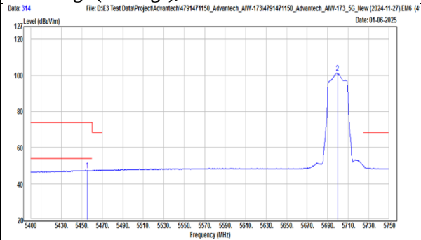
TX, 802.11be(EHT20) (Ch 140) Band Edge (Peak), Vertical
