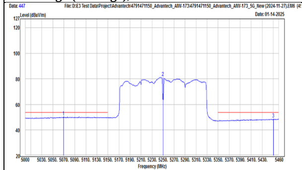
TX, 802.11ac(VHT160) (Ch 50) Band Edge (Peak), Horizontal
