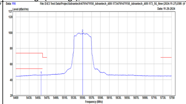
TX, 802.11be(EHT40) (Ch 110) Band Edge (Peak), Vertical
