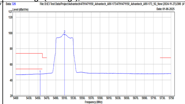
TX, 802.11be(EHT40) (Ch 102) Band Edge (Peak), Vertical
