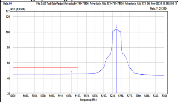
TX, 802.11be(EHT20) (Ch 48) Band Edge (Peak), Vertical
