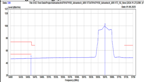
TX, 802.11be(EHT40) (Ch 134) Band Edge (Peak), Vertical
