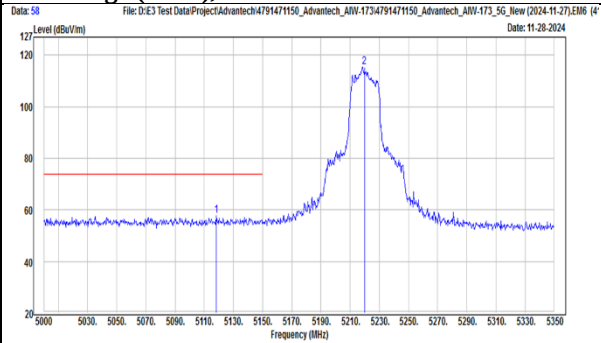
TX, 802.11be(EHT20) (Ch 44) Band Edge (Peak), Vertical
