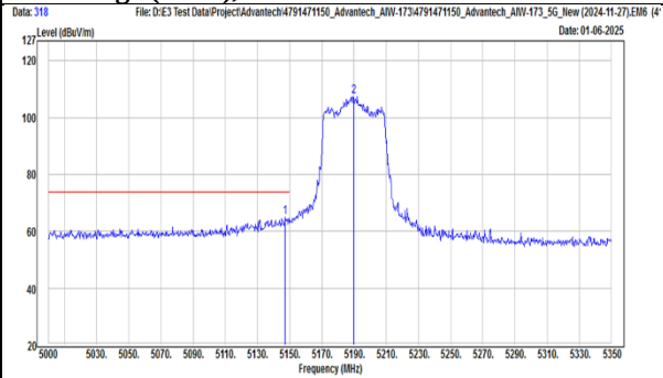
TX, 802.11be(EHT40) (Ch 38) Band Edge (Peak), Vertical
