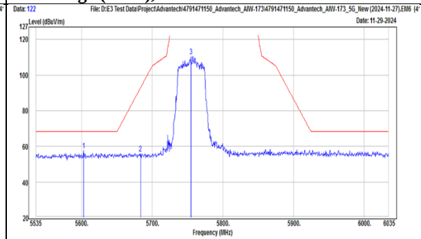
TX, 802.11be(EHT40) (Ch 151) Band Edge (Peak), Vertical
