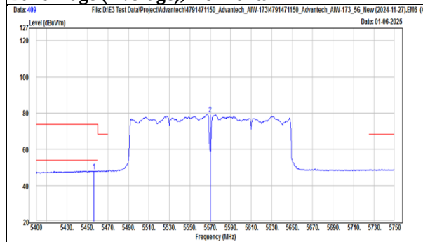
TX, 802.11ac(VHT160) (Ch 114) Band Edge (Peak), Horizontal
