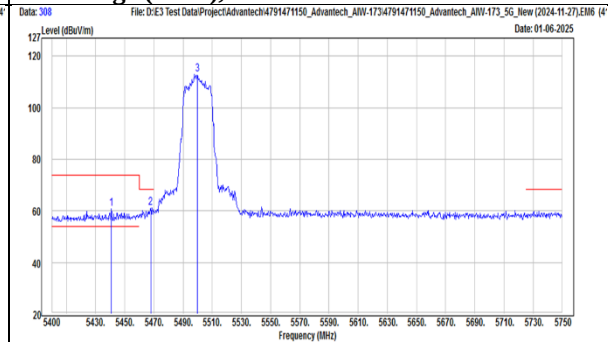
TX, 802.11be(EHT20) (Ch 100) Band Edge (Peak), Vertical
