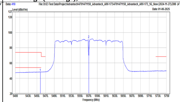
TX, 802.11ac(VHT160) (Ch 114) Band Edge (Peak), Vertical
