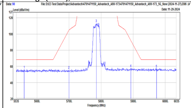
TX, 802.11be(EHT20) (Ch 157) Band Edge (Peak), Vertical
