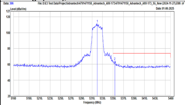
TX, 802.11be(EHT20) (Ch 64) Band Edge (Peak), Vertical
