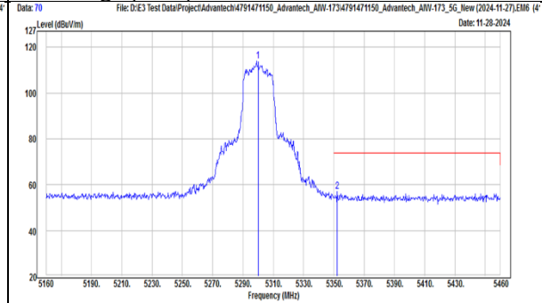
TX, 802.11be(EHT20) (Ch 60) Band Edge (Peak), Vertical
