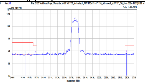
TX, 802.11be(EHT20) (Ch 116) Band Edge (Peak), Vertical
