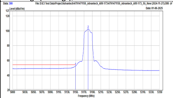
TX, 802.11be(EHT20) (Ch 36) Band Edge (Peak), Vertical
