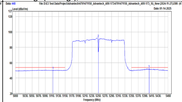
TX, 802.11ac(VHT160) (Ch 50) Band Edge (Peak), Vertical
