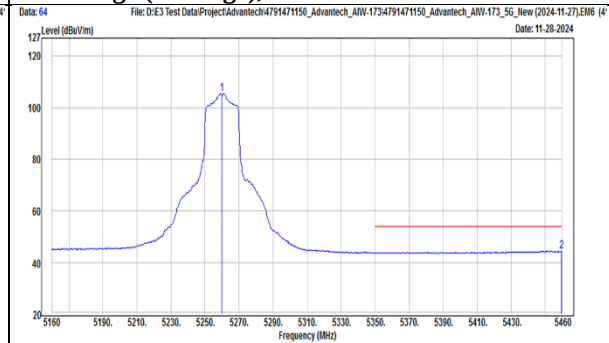
TX, 802.11be(EHT20) (Ch 52) Band Edge (Peak), Vertical
