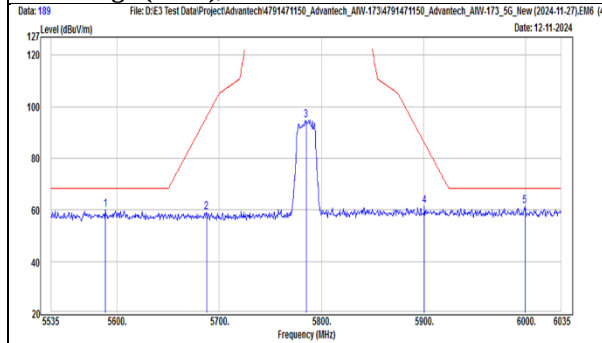
TX, 802.11ac(VHT20) (Ch 157) Band Edge (Peak), Horizontal
