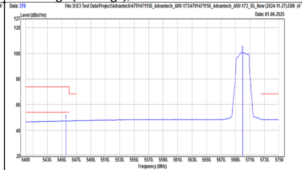
TX, 802.11ac(VHT20) (Ch 140) Band Edge (Peak), Vertical
