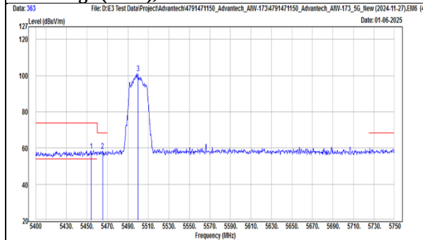
TX, 802.11ac(VHT20) (Ch 100) Band Edge (Peak), Horizontal
