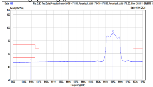
TX, 802.11ac(VHT40) (Ch 134) Band Edge (Peak), Horizontal
