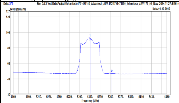
TX, 802.11ac(VHT40) (Ch 62) Band Edge (Peak), Horizontal
