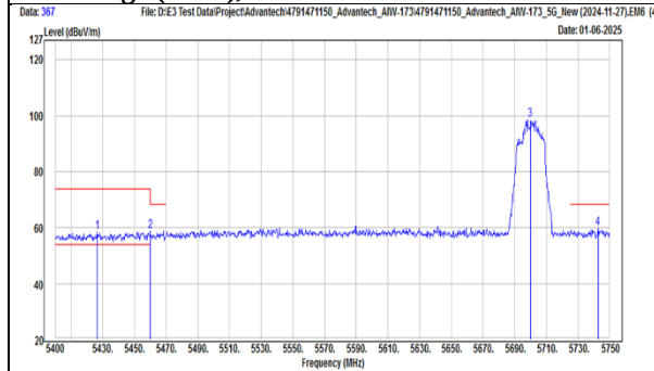
TX, 802.11ac(VHT20) (Ch 140) Band Edge (Peak), Horizontal
