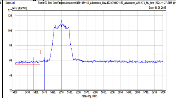
TX, 802.11ac(VHT40) (Ch 102) Band Edge (Peak), Vertical
