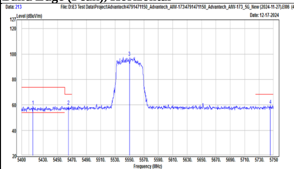
TX, 802.11ac(VHT40) (Ch 110) Band Edge (Peak), Horizontal
