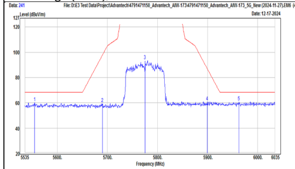
TX, 802.11ac(VHT80) (Ch 155) Band Edge (Peak), Horizontal
