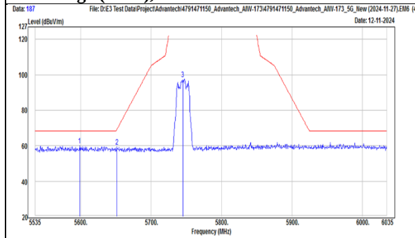
TX, 802.11ac(VHT20) (Ch 149) Band Edge (Peak), Horizontal
