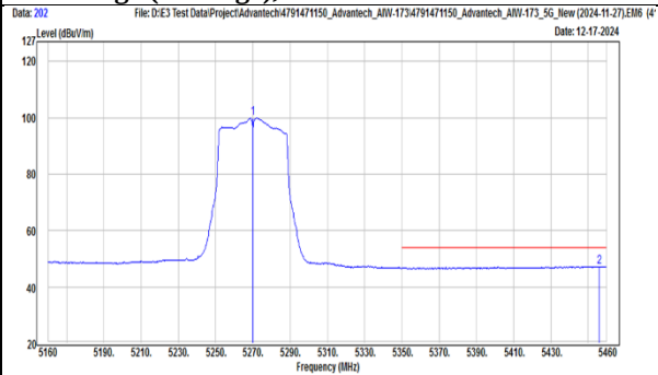
TX, 802.11ac(VHT40) (Ch 54) Band Edge (Peak), Vertical
