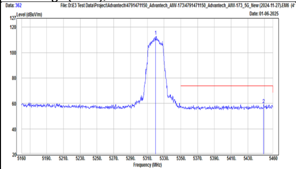
TX, 802.11ac(VHT20) (Ch 64) Band Edge (Peak), Vertical
