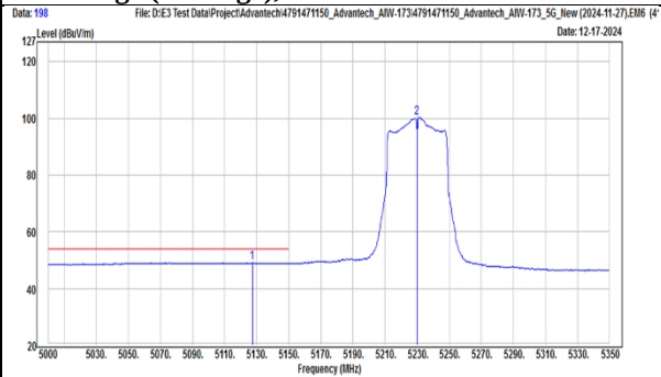
TX, 802.11ac(VHT40) (Ch 46) Band Edge (Peak), Vertical
