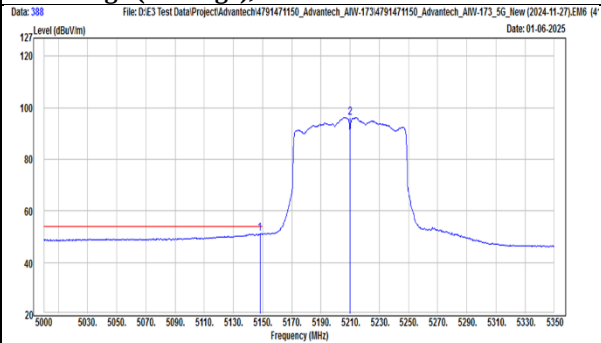
TX, 802.11ac(VHT80) (Ch 42) Band Edge (Peak), Vertical
