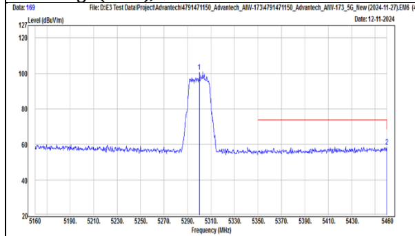
TX, 802.11ac(VHT20) (Ch 60) Band Edge (Peak), Horizontal
