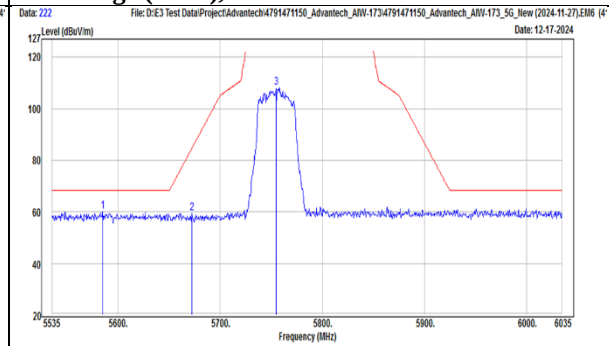
TX, 802.11ac(VHT40) (Ch 151) Band Edge (Peak), Vertical
