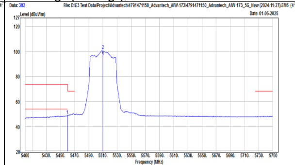
TX, 802.11ac(VHT40) (Ch 102) Band Edge (Peak), Vertical
