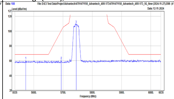
TX, 802.11ac(VHT20) (Ch 149) Band Edge (Peak), Vertical
