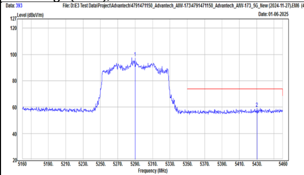
TX, 802.11ac(VHT80) (Ch 58) Band Edge (Peak), Horizontal
