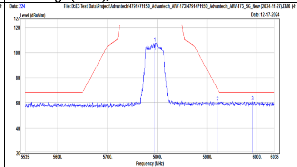
TX, 802.11ac(VHT40) (Ch 159) Band Edge (Peak), Vertical
