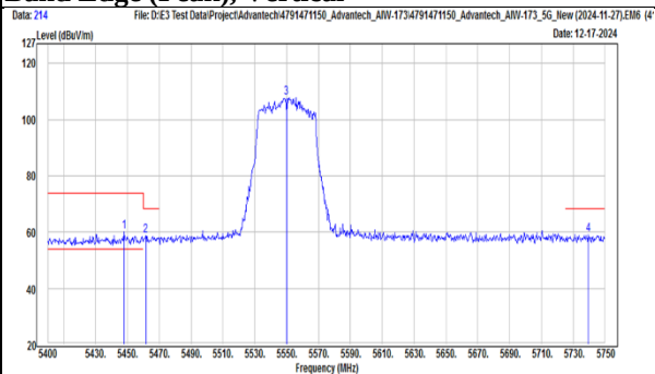
TX, 802.11ac(VHT40) (Ch 110) Band Edge (Peak), Vertical
