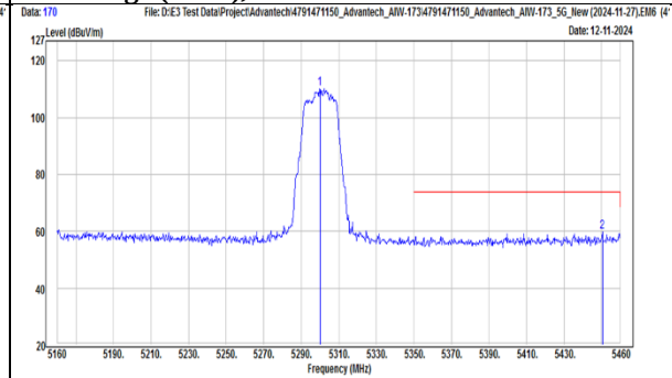
TX, 802.11ac(VHT20) (Ch 60) Band Edge (Peak), Vertical
