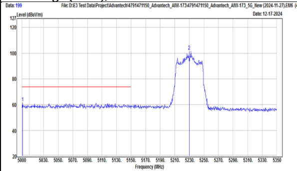
TX, 802.11ac(VHT40) (Ch 46) Band Edge (Peak), Horizontal
