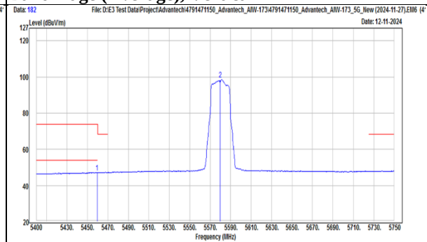
TX, 802.11ac(VHT20) (Ch 116) Band Edge (Peak), Vertical
