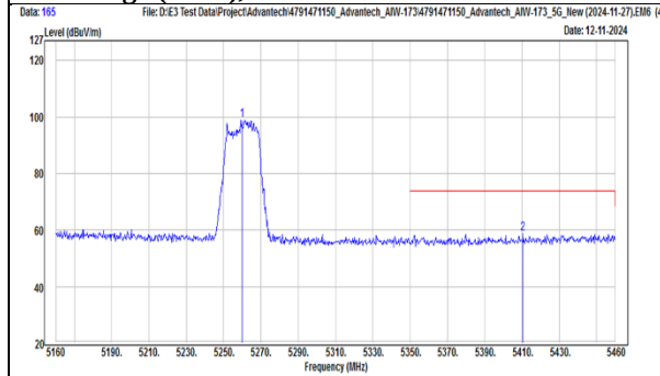
TX, 802.11ac(VHT20) (Ch 52) Band Edge (Peak), Horizontal
