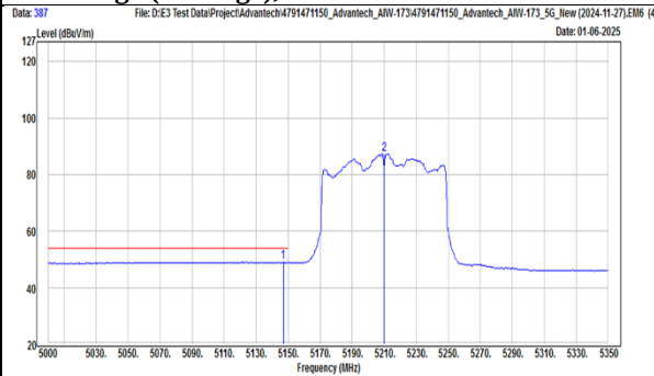
TX, 802.11ac(VHT80) (Ch 42) Band Edge (Peak), Horizontal
