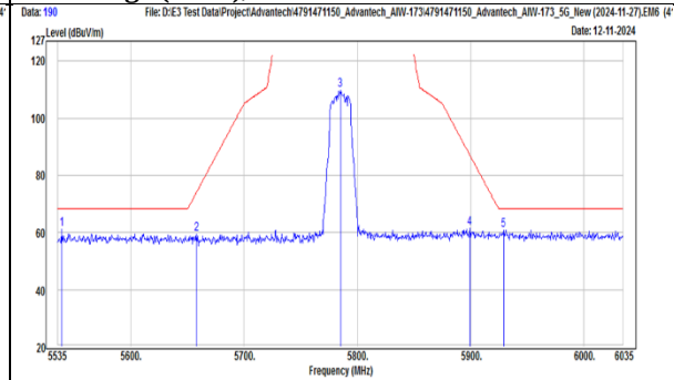
TX, 802.11ac(VHT20) (Ch 157) Band Edge (Peak), Vertical
