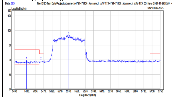
TX, 802.11ac(VHT80) (Ch 106) Band Edge (Peak), Horizontal
