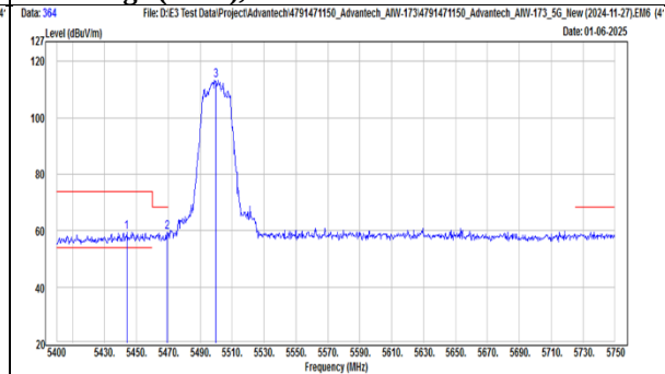
TX, 802.11ac(VHT20) (Ch 100) Band Edge (Peak), Vertical
