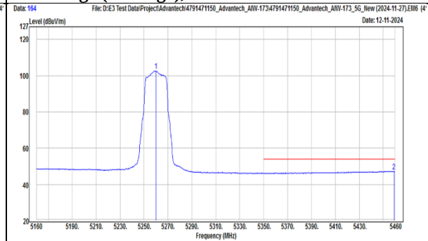
TX, 802.11ac(VHT20) (Ch 52) Band Edge (Peak), Vertical
