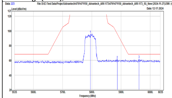
TX, 802.11ac(VHT40) (Ch 159) Band Edge (Peak), Horizontal
