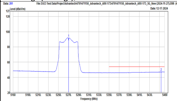
TX, 802.11ac(VHT40) (Ch 54) Band Edge (Peak), Horizontal
