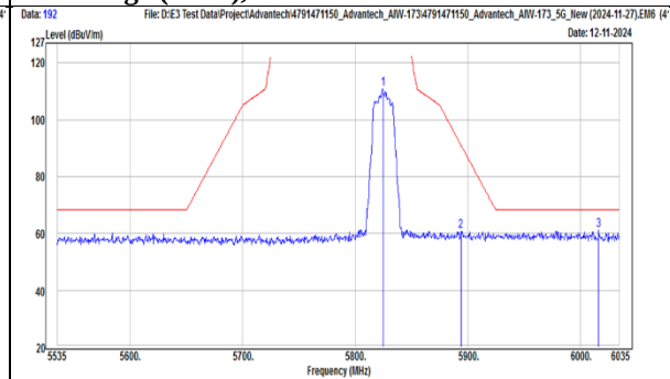
TX, 802.11ac(VHT20) (Ch 165) Band Edge (Peak), Vertical
