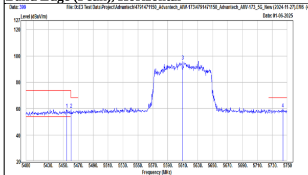
TX, 802.11ac(VHT80) (Ch 122) Band Edge (Peak), Horizontal
