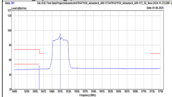
TX, 802.11ac(VHT40) (Ch 102) Band Edge (Peak), Horizontal
