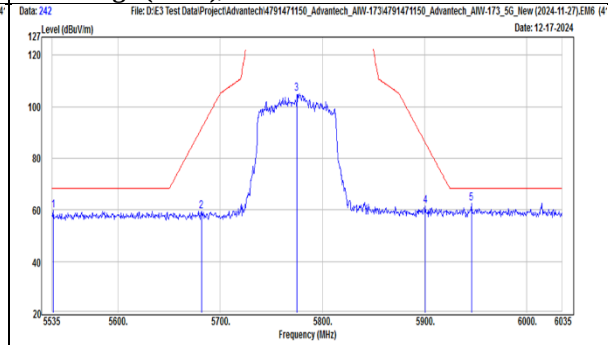
TX, 802.11ac(VHT80) (Ch 155) Band Edge (Peak), Vertical
