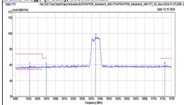
TX, 802.11ac(VHT20) (Ch 116) Band Edge (Peak), Horizontal
