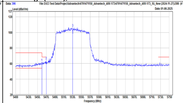
TX, 802.11ac(VHT80) (Ch 106) Band Edge (Peak), Vertical
