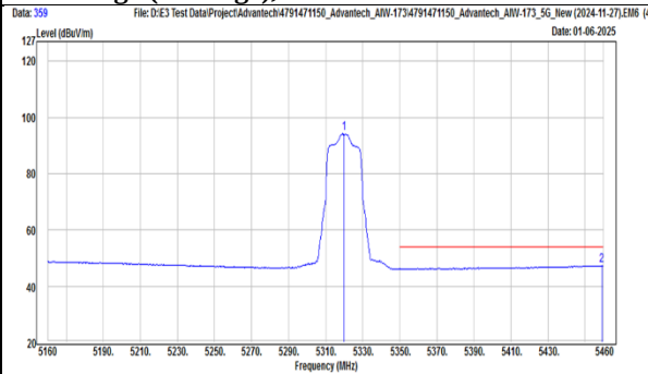
TX, 802.11ac(VHT20) (Ch 64) Band Edge (Peak), Horizontal
