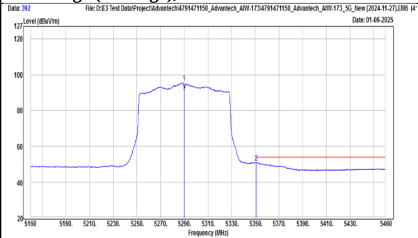
TX, 802.11ac(VHT80) (Ch 58) Band Edge (Peak), Vertical
