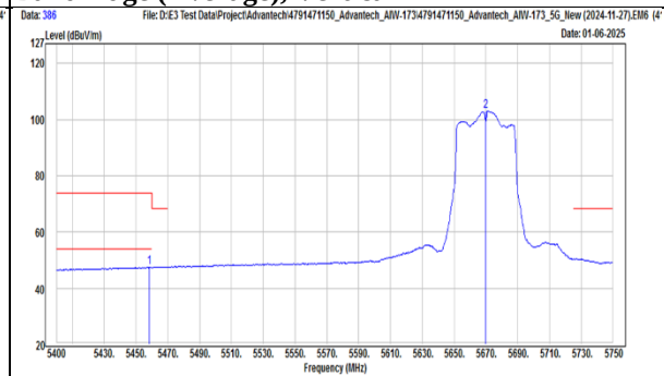
TX, 802.11ac(VHT40) (Ch 134) Band Edge (Peak), Vertical
