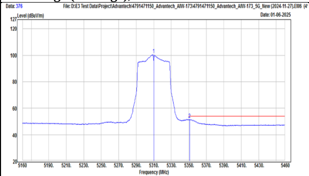
TX, 802.11ac(VHT40) (Ch 62) Band Edge (Peak), Vertical
