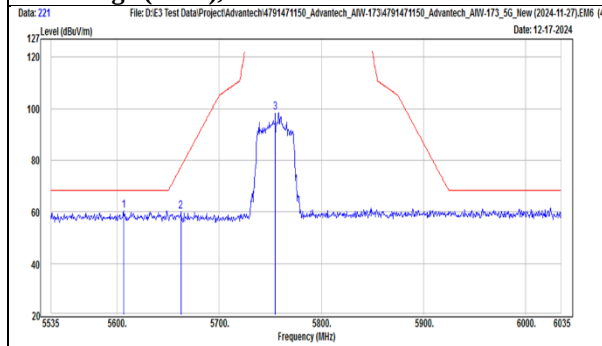
TX, 802.11ac(VHT40) (Ch 151) Band Edge (Peak), Horizontal
