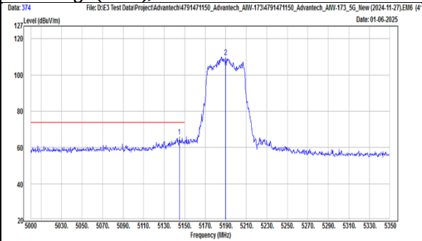
TX, 802.11ac(VHT40) (Ch 38) Band Edge (Peak), Vertical
