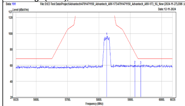
TX, 802.11ac(VHT20) (Ch 165) Band Edge (Peak), Horizontal
