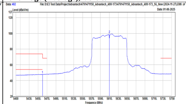
TX, 802.11ac(VHT80) (Ch 122) Band Edge (Peak), Vertical
