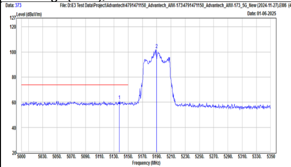
TX, 802.11ac(VHT40) (Ch 38) Band Edge (Peak), Horizontal
