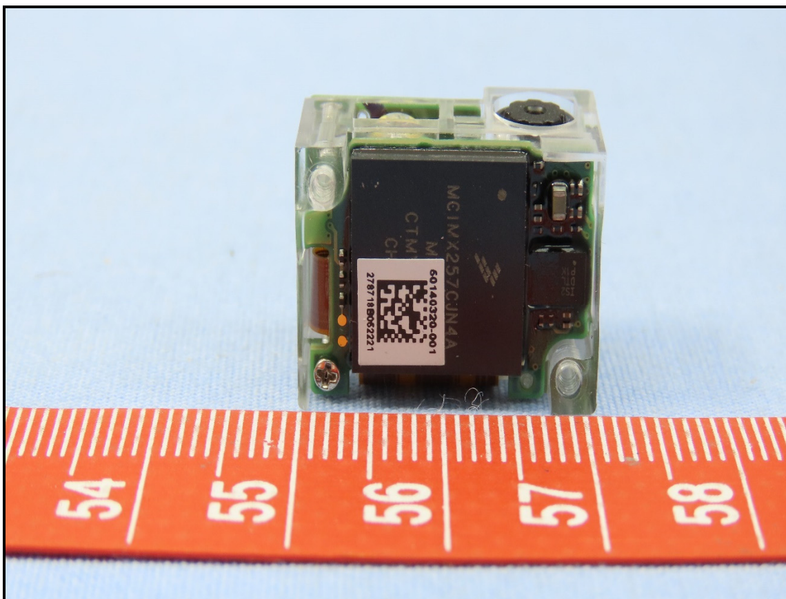
Extension Modules- Barcode scanner (70° ) (Brand: ADVANTECH, Model: AIM-EXT0-0041 (70 degree)) (option)
