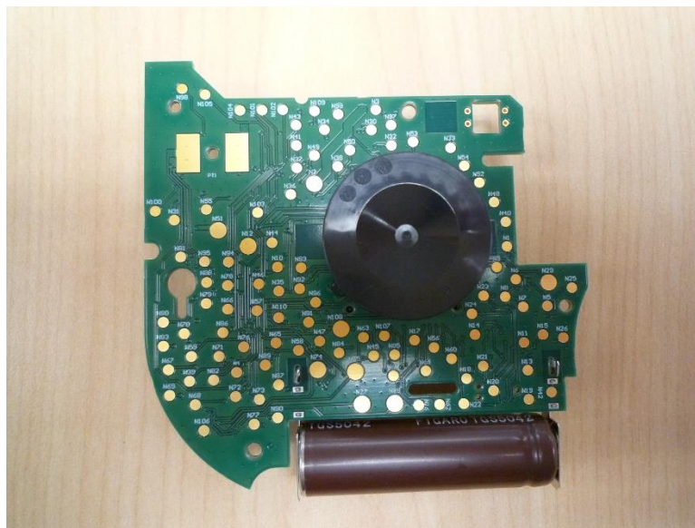
Figure 2 Back view Sensor PCB
