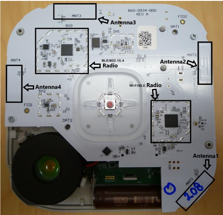
Figure 3 Front view Radio PCB
