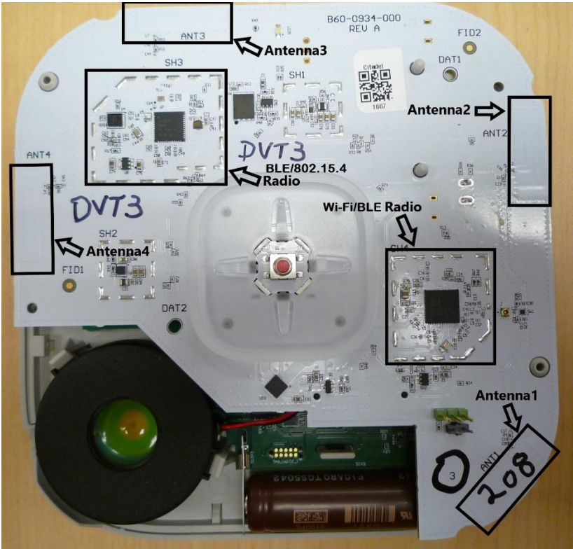
Figure 7 Top View Radio PCB
