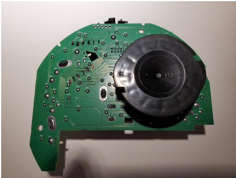
Figure 5 Bottom Layer PCB back view
