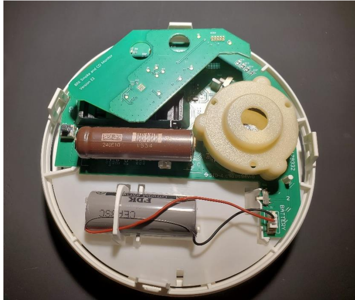
Figure 1 Top view
