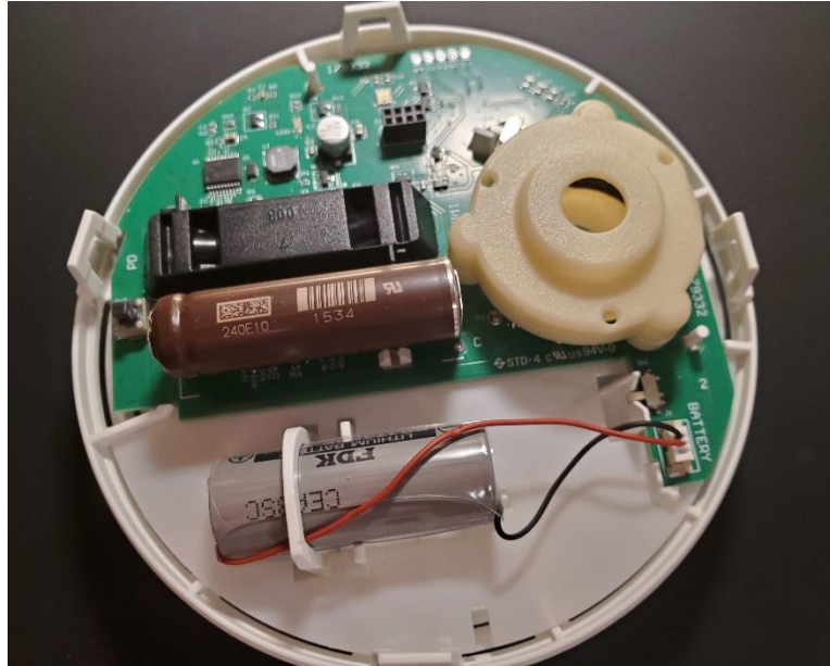
Figure 2 Top view without top layer PCB
