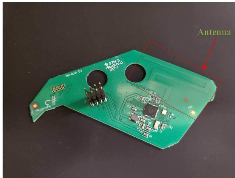
Figure 3 Top layer PCB back side view
