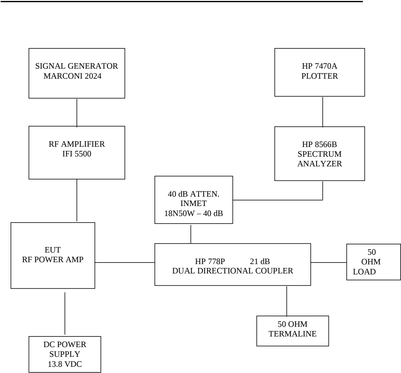
FIGURE 2: Block Diagram (Power Input/Output tests)
