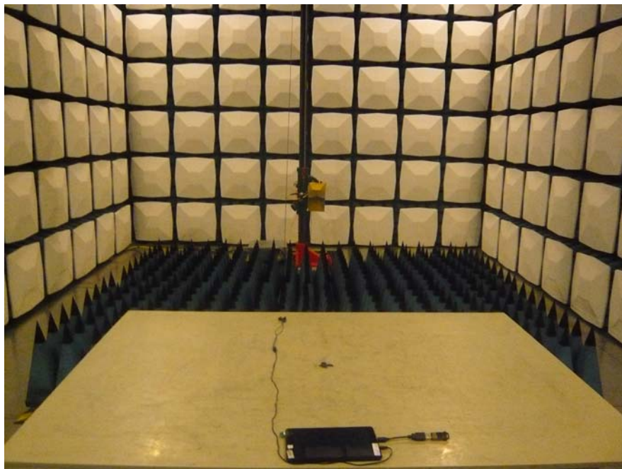
Radiated Emission –Rear View (Above 1 GHz) -USB Playing
