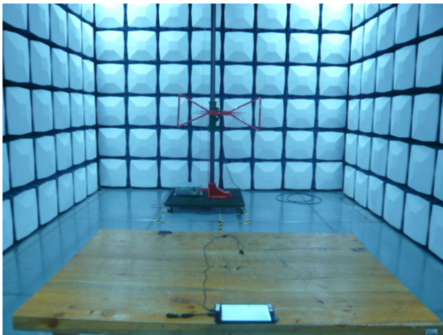
Radiated Emissions –Rear View (Below 1GHz) -USB Playing
