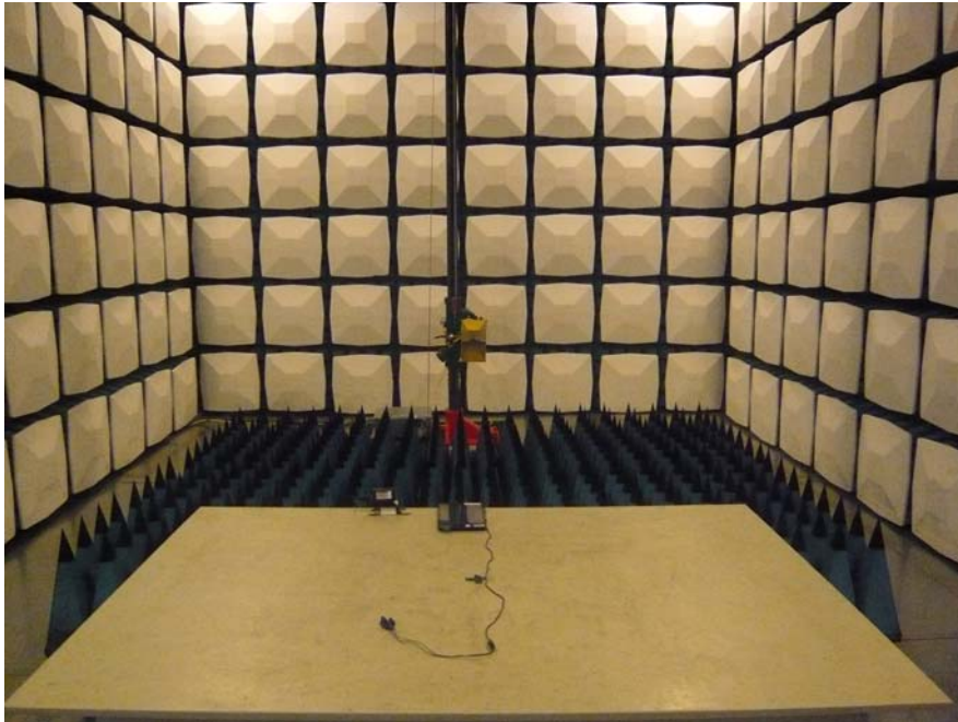
Radiated Emission –Front View (Above 1 GHz)-Charging & Playing
