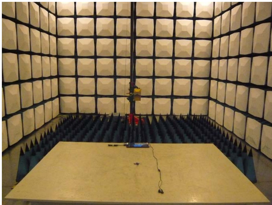
Radiated Emission –Front View (Above 1 GHz)-USB Playing
