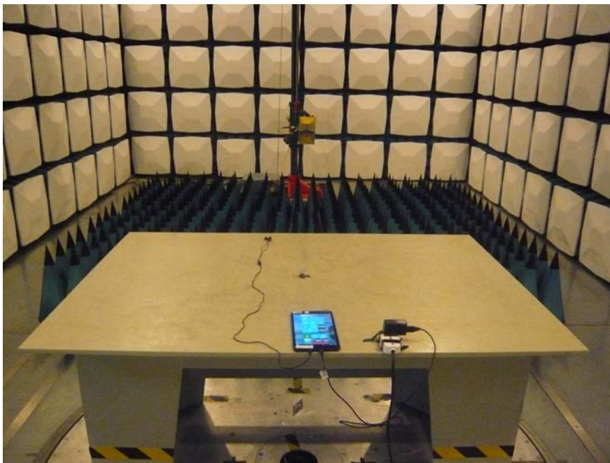
Radiated Emission –Rear View (Above 1 GHz) -Charging & Playing
