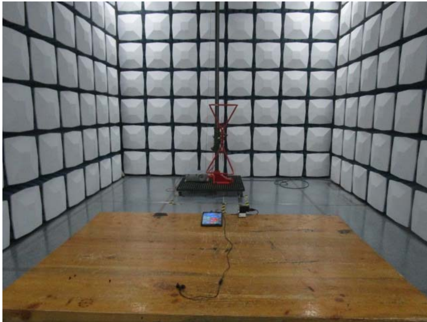
Radiated Emissions –Front View (Below 1GHz)-Charging & Playing
