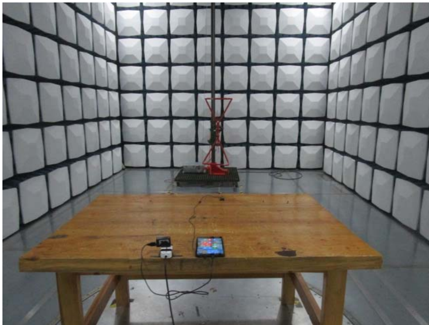
Radiated Emissions –Rear View (Below 1GHz) -Charging & Playing
