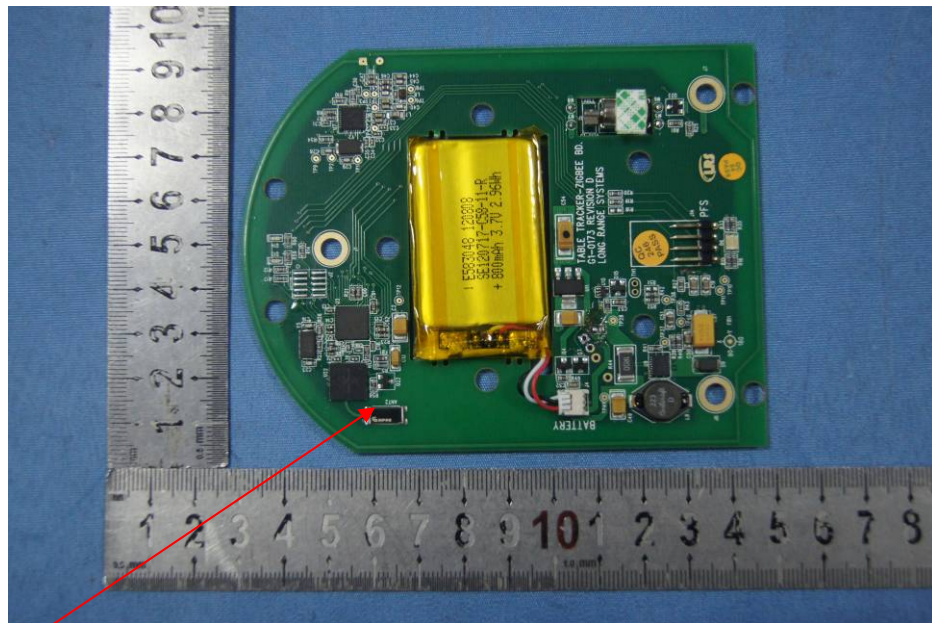
Antenna for Zigbee
