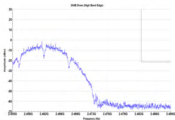
2462MHz (Upper Band Edge, Port 2)
