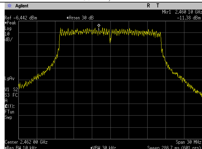
2462MHz, Port 1
