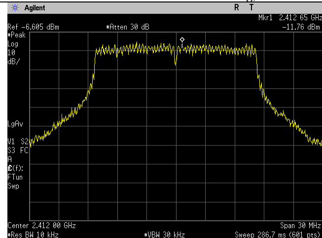
2412MHz, Port 1
