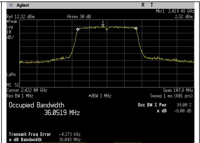
2422MHz 99% Bandwidth
