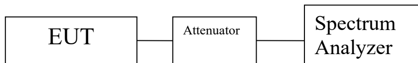
Figure 10. Block Diagram, Peak Power Spectral Density Test Setup
