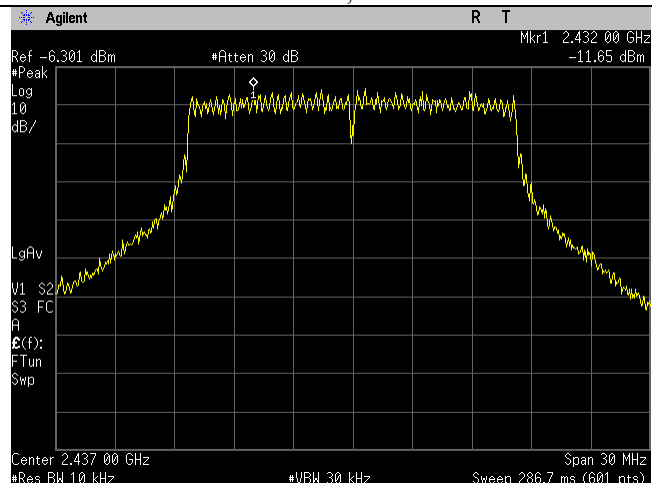
2437MHz, Port 2
