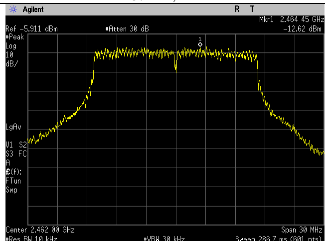
2462MHz, Port 2
