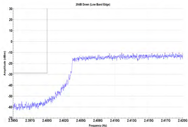
2412MHz (Lower Band Edge, Port 1)
