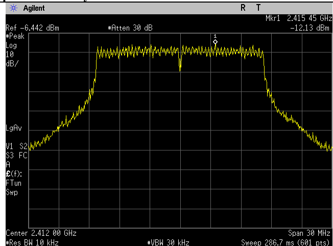
2412MHz, Port 2
