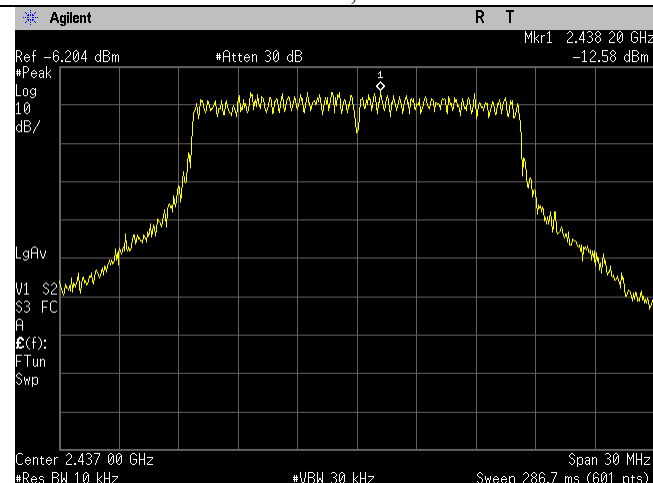
2437MHz, Port 1
