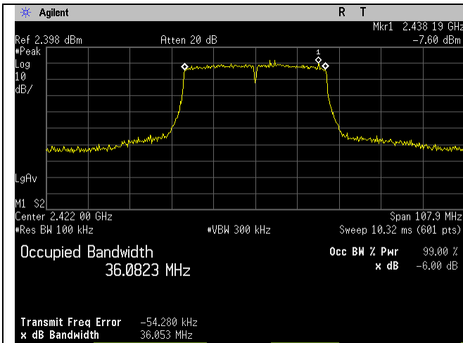
2422MHz 6dB Bandwidth
