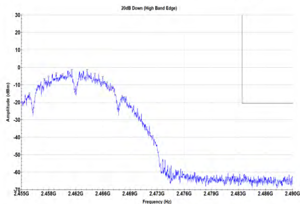
2462MHz (Upper Band Edge, Port 1)
