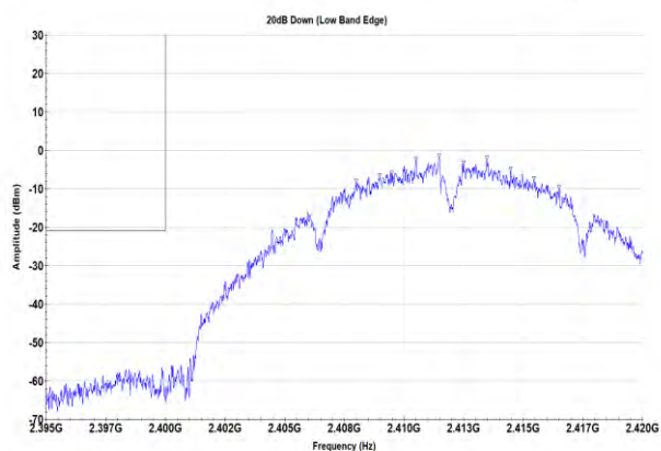
2412MHz (Lower Band Edge, Port 2)
