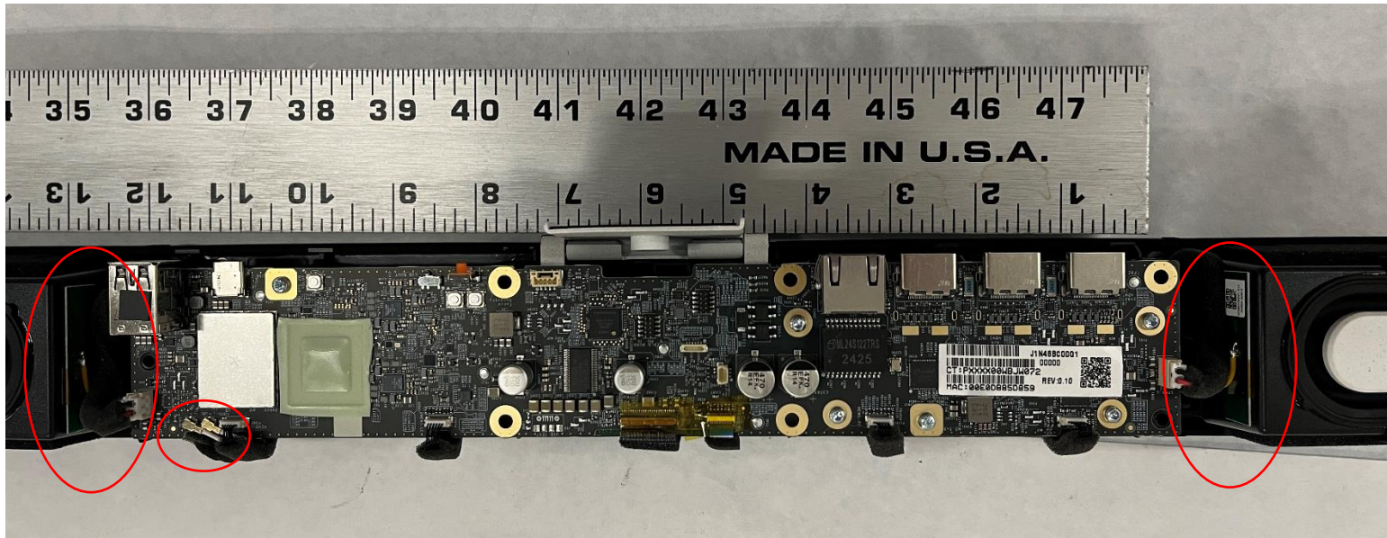
Antenna and Antenna Connector Location
