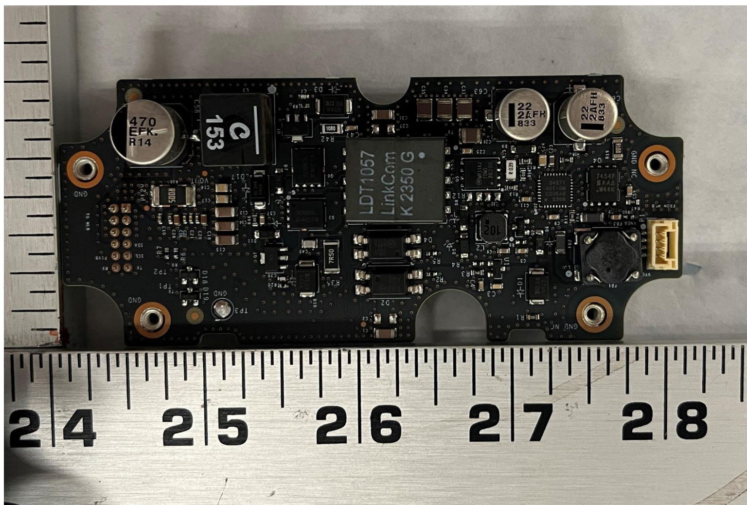
Daughter Board Front Side
