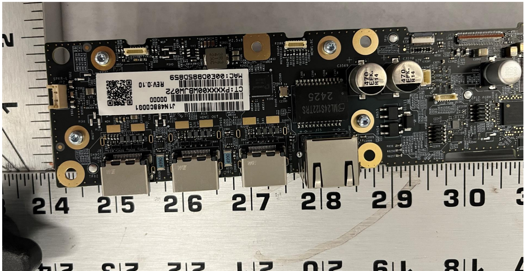
PCB Close Up with on Connector Side of Board
