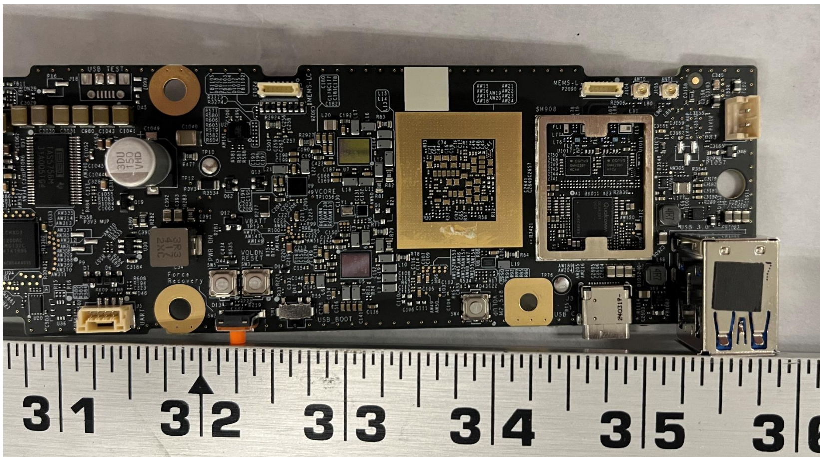
PCB Close Up with Shielding Over RF Circuitry Removed
