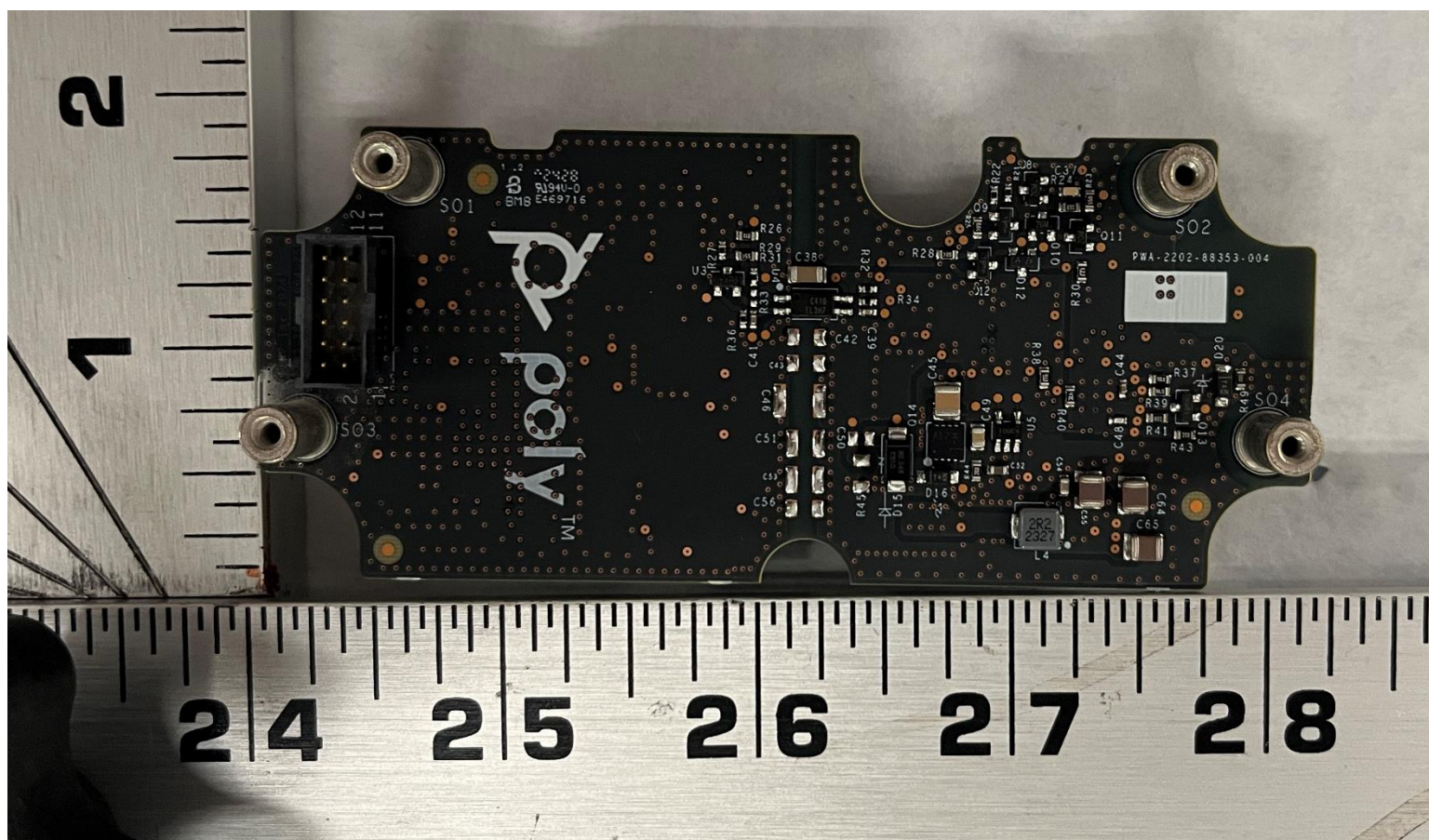
Daughter Board Back Side
