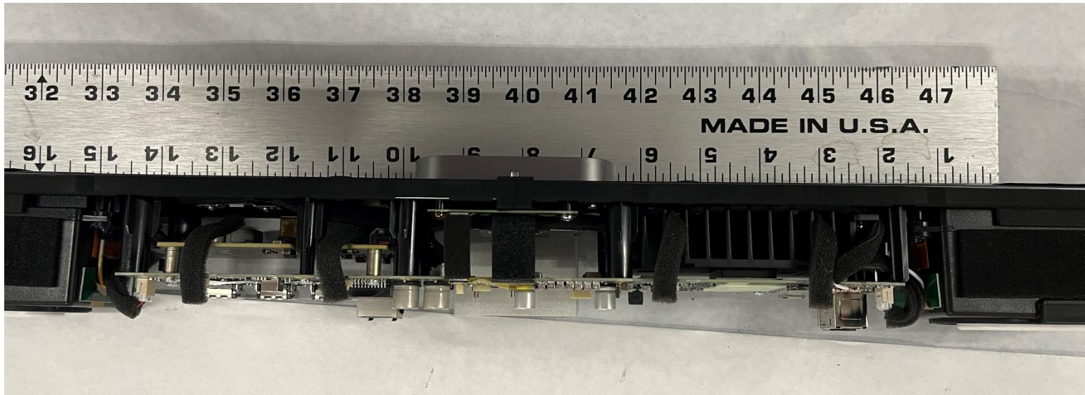
Antenna Location (Edge 2 View)
