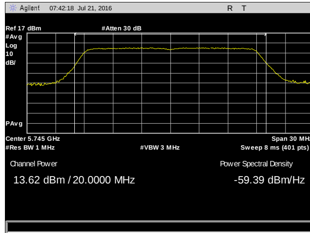
Plot 9. Conducted Output Power, 802.11n 20 MHz, 5745 MHz, Chain 0
