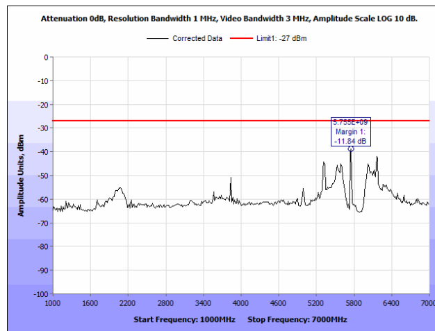
Plot 29. Radiated Spurious Emissions, 802.11n 20 MHz, 5745 MHz, Both Chains, 1 GHz – 7 GHz
