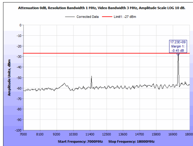
Plot 21. Radiated Spurious Emissions, 802.11a 20 MHz, 5745 MHz, Both Chains, 7 GHz – 18 GHz
