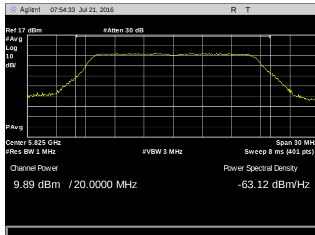
Plot 5. Conducted Output Power, 802.11a 20 MHz, 5825 MHz, Chain 0
