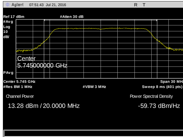
Plot 3. Conducted Output Power, 802.11a 20 MHz, 5745 MHz, Chain 0
