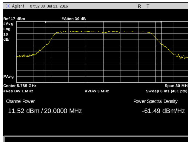
Plot 4. Conducted Output Power, 802.11a 20 MHz, 5785 MHz, Chain 0
