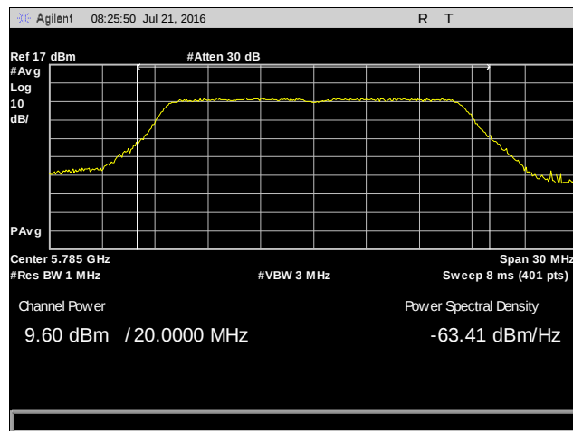
Plot 7. Conducted Output Power, 802.11a 20 MHz, 5785 MHz, Chain 1
