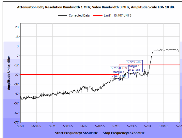
Plot 47. Radiated Band Edge, 802.11n 40 MHz, 5755 MHz, Both Chains
