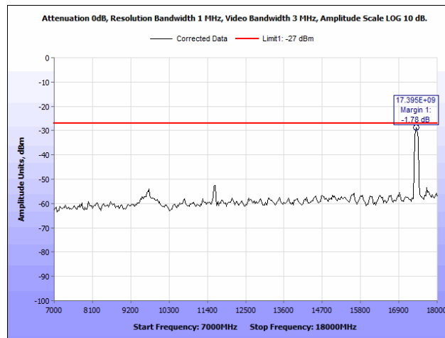
Plot 42. Radiated Spurious Emissions, 802.11n 40 MHz, 5795 MHz, Both Chains, 7 GHz – 18 GHz
