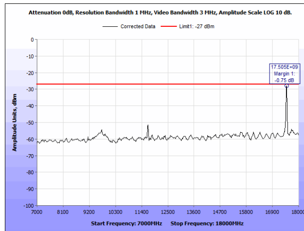
Plot 27. Radiated Spurious Emissions, 802.11a 20 MHz, 5825 MHz, Both Chains, 7 GHz – 18 GHz
