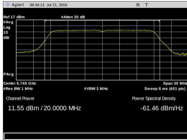
Plot 12. Conducted Output Power, 802.11n 20 MHz, 5745 MHz, Chain 1
