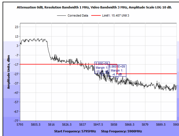
Plot 48. Radiated Band Edge, 802.11n 40 MHz, 5795 MHz, Both Chains
