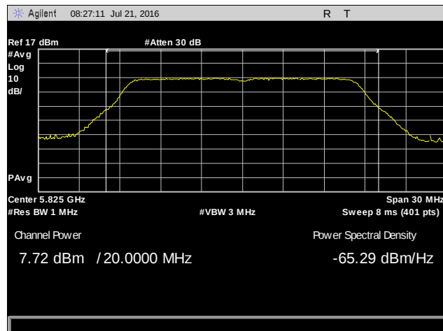
Plot 8. Conducted Output Power, 802.11a 20 MHz, 5825 MHz, Chain 1
