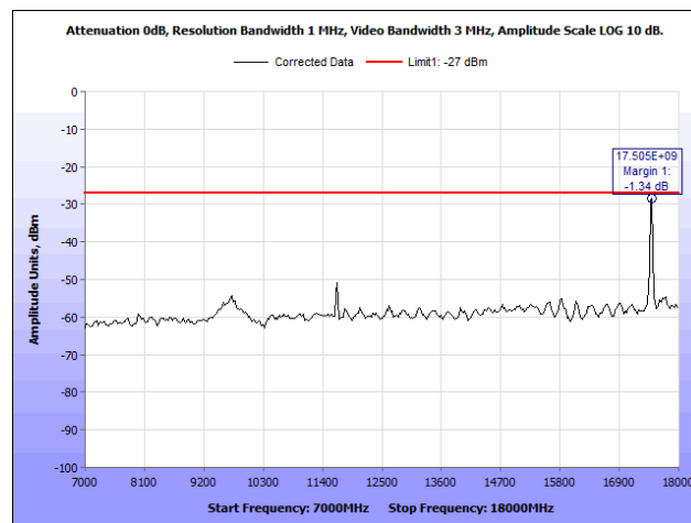
Plot 36. Radiated Spurious Emissions, 802.11n 20 MHz, 5825 MHz, Both Chains, 7 GHz – 18 GHz
