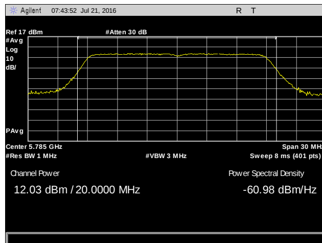
Plot 10. Conducted Output Power, 802.11n 20 MHz, 5785 MHz, Chain 0
