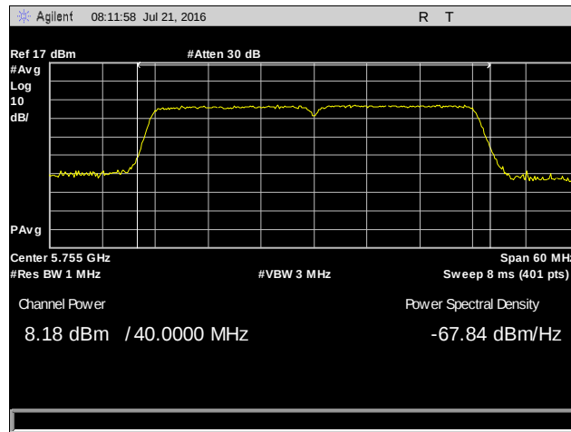
Plot 17. Conducted Output Power, 802.11n 40 MHz, 5755 MHz, Chain 1
