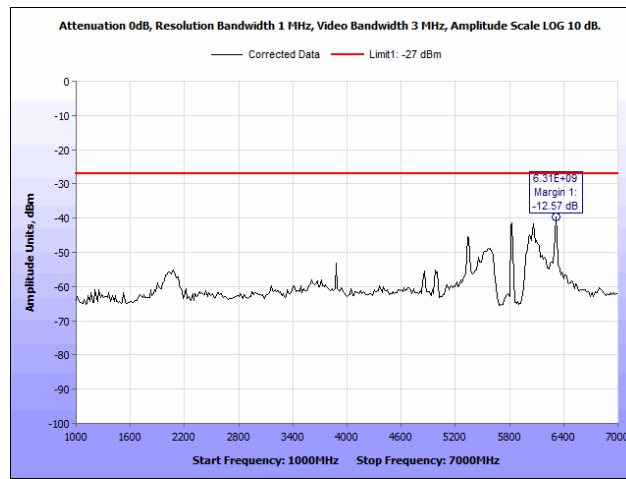
Plot 26. Radiated Spurious Emissions, 802.11a 20 MHz, 5825 MHz, Both Chains, 1 GHz – 7 GHz
