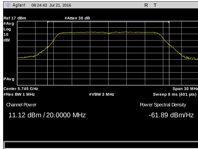
Plot 6. Conducted Output Power, 802.11a 20 MHz, 5745 MHz, Chain 1
