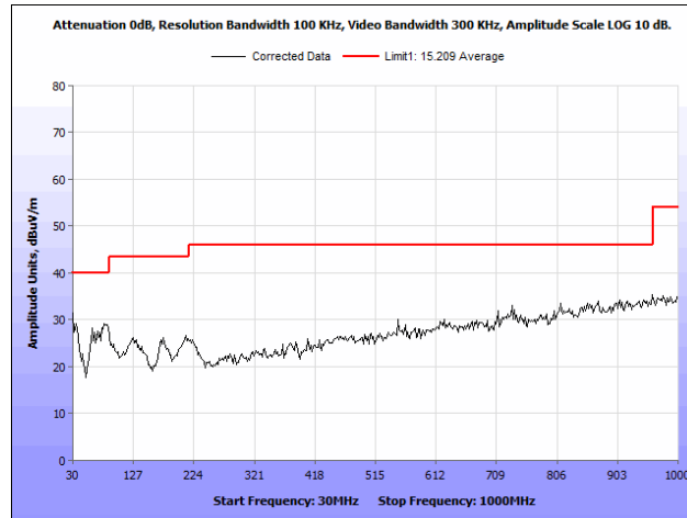
Plot 31. Radiated Spurious Emissions, 802.11n 20 MHz, 5785 MHz, Both Chains, 30 MHz – 1 GHz
