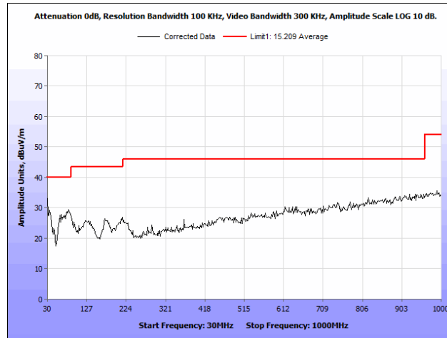
Plot 40. Radiated Spurious Emissions, 802.11n 40 MHz, 5795 MHz, Both Chains, 30 MHz – 1 GHz
