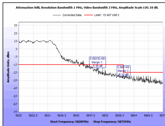
Plot 46. Radiated Band Edge, 802.11n 20 MHz, 5825 MHz, Both Chains
