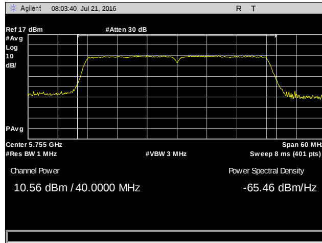
Plot 15. Conducted Output Power, 802.11n 40 MHz, 5755 MHz, Chain 0
