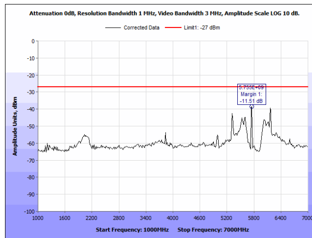
Plot 20. Radiated Spurious Emissions, 802.11a 20 MHz, 5745 MHz, Both Chains, 1 GHz – 7 GHz
