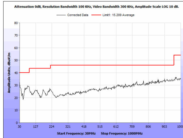
Plot 34. Radiated Spurious Emissions, 802.11n 20 MHz, 5825 MHz, Both Chains, 30 MHz – 1 GHz
