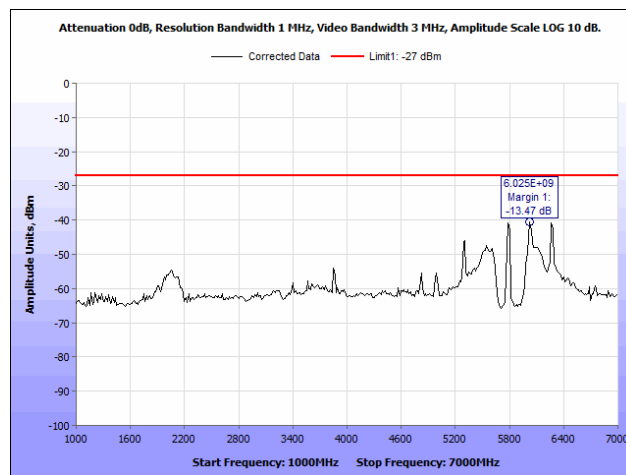
Plot 23. Radiated Spurious Emissions, 802.11a 20 MHz, 5785 MHz, Both Chains, 1 GHz – 7 GHz
