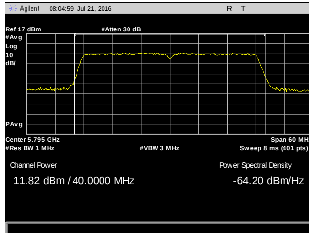
Plot 16. Conducted Output Power, 802.11n 40 MHz, 5795 MHz, Chain 0
