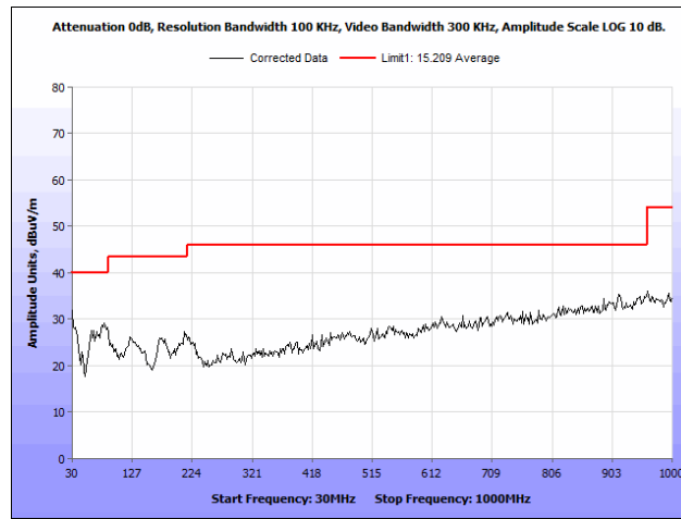
Plot 37. Radiated Spurious Emissions, 802.11n 40 MHz, 5755 MHz, Both Chains, 30 MHz – 1 GHz
