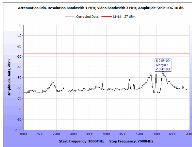
Plot 41. Radiated Spurious Emissions, 802.11n 40 MHz, 5795 MHz, Both Chains, 1 GHz – 7 GHz
