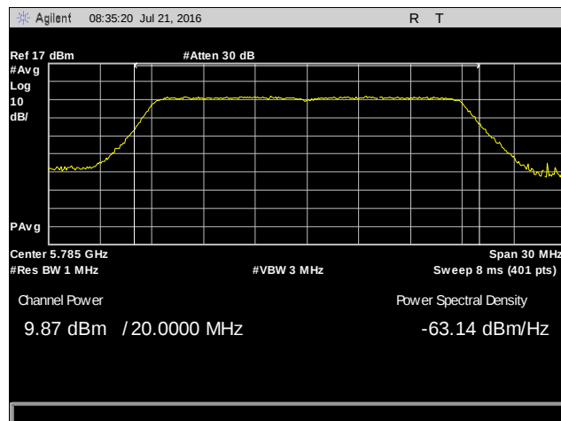
Plot 13. Conducted Output Power, 802.11n 20 MHz, 5785 MHz, Chain 1
