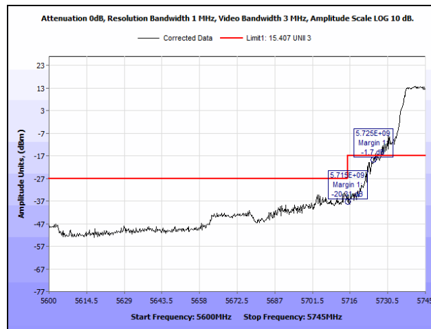
Plot 43. Radiated Band Edge, 802.11a 20 MHz, 5745 MHz, Both Chains
