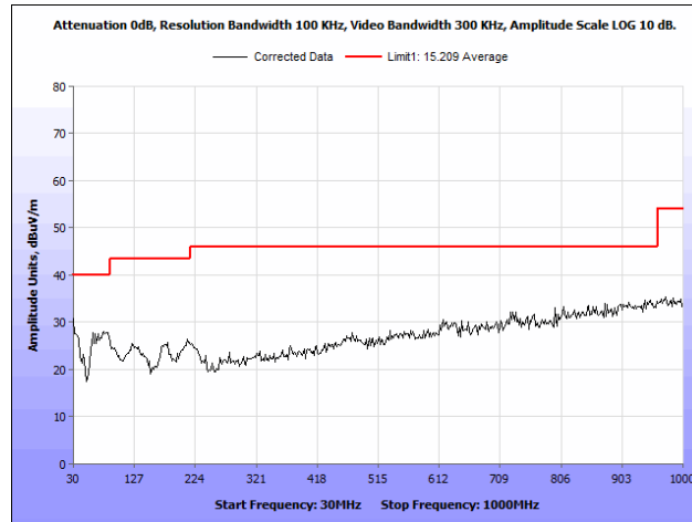
Plot 22. Radiated Spurious Emissions, 802.11a 20 MHz, 5785 MHz, Both Chains, 30 MHz – 1 GHz
