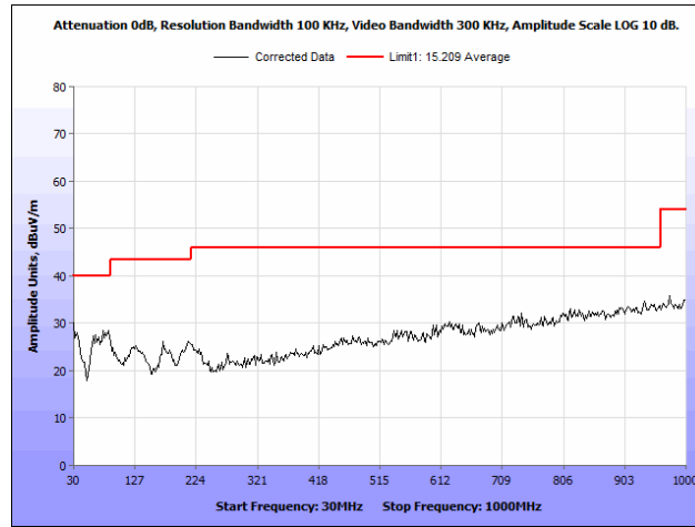
Plot 19. Radiated Spurious Emissions, 802.11a 20 MHz, 5745 MHz, Both Chains, 30 MHz – 1 GHz
