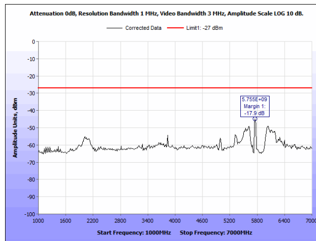
Plot 38. Radiated Spurious Emissions, 802.11n 40 MHz, 5755 MHz, Both Chains, 1 GHz – 7 GHz
