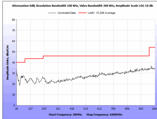
Plot 25. Radiated Spurious Emissions, 802.11a 20 MHz, 5825 MHz, Both Chains, 30 MHz – 1 GHz
