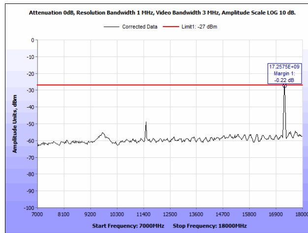
Plot 30. Radiated Spurious Emissions, 802.11n 20 MHz, 5745 MHz, Both Chains, 7 GHz – 18 GHz
