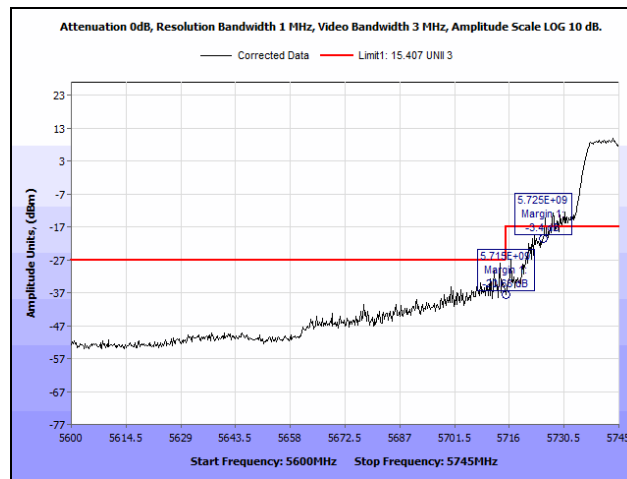
Plot 45. Radiated Band Edge, 802.11n 20 MHz, 5745 MHz, Both Chains
