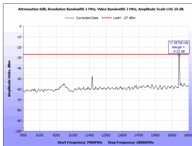
Plot 24. Radiated Spurious Emissions, 802.11a 20 MHz, 5785 MHz, Both Chains, 7 GHz – 18 GHz
