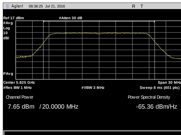
Plot 14. Conducted Output Power, 802.11n 20 MHz, 5825 MHz, Chain 1
