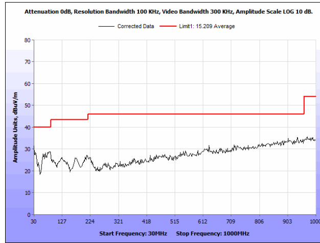
Plot 28. Radiated Spurious Emissions, 802.11n 20 MHz, 5745 MHz, Both Chains, 30 MHz – 1 GHz
