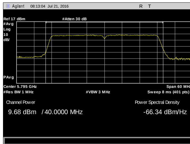
Plot 18. Conducted Output Power, 802.11n 40 MHz, 5795 MHz, Chain 1
