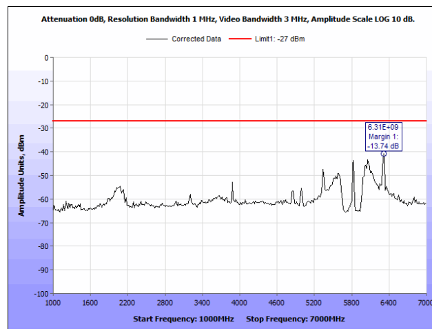
Plot 35. Radiated Spurious Emissions, 802.11n 20 MHz, 5825 MHz, Both Chains, 1 GHz – 7 GHz
