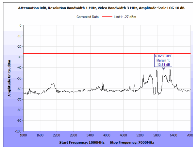
Plot 32. Radiated Spurious Emissions, 802.11n 20 MHz, 5785 MHz, Both Chains, 1 GHz – 7 GHz
