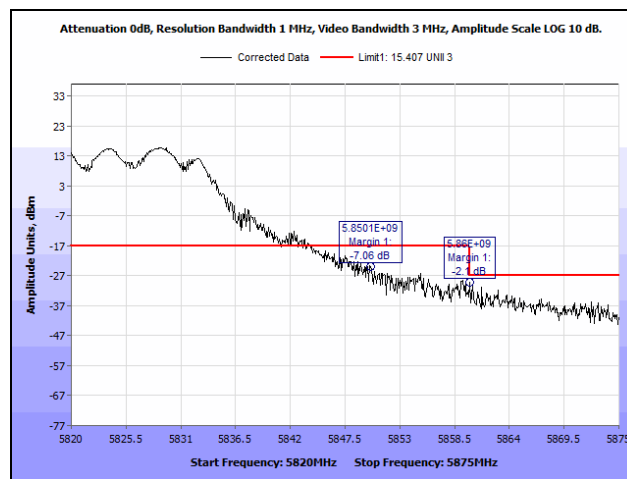
Plot 44. Radiated Band Edge, 802.11a 20 MHz, 5825 MHz, Both Chains
