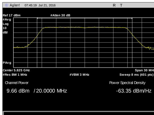
Plot 11. Conducted Output Power, 802.11n 20 MHz, 5825 MHz, Chain 0
