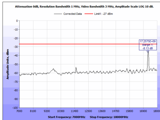
Plot 39. Radiated Spurious Emissions, 802.11n 40 MHz, 5755 MHz, Both Chains, 7 GHz – 18 GHz
