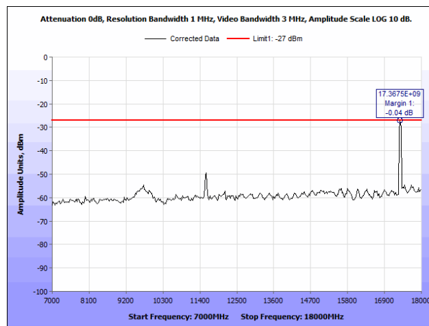
Plot 33. Radiated Spurious Emissions, 802.11n 20 MHz, 5785 MHz, Both Chains, 7 GHz – 18 GHz
