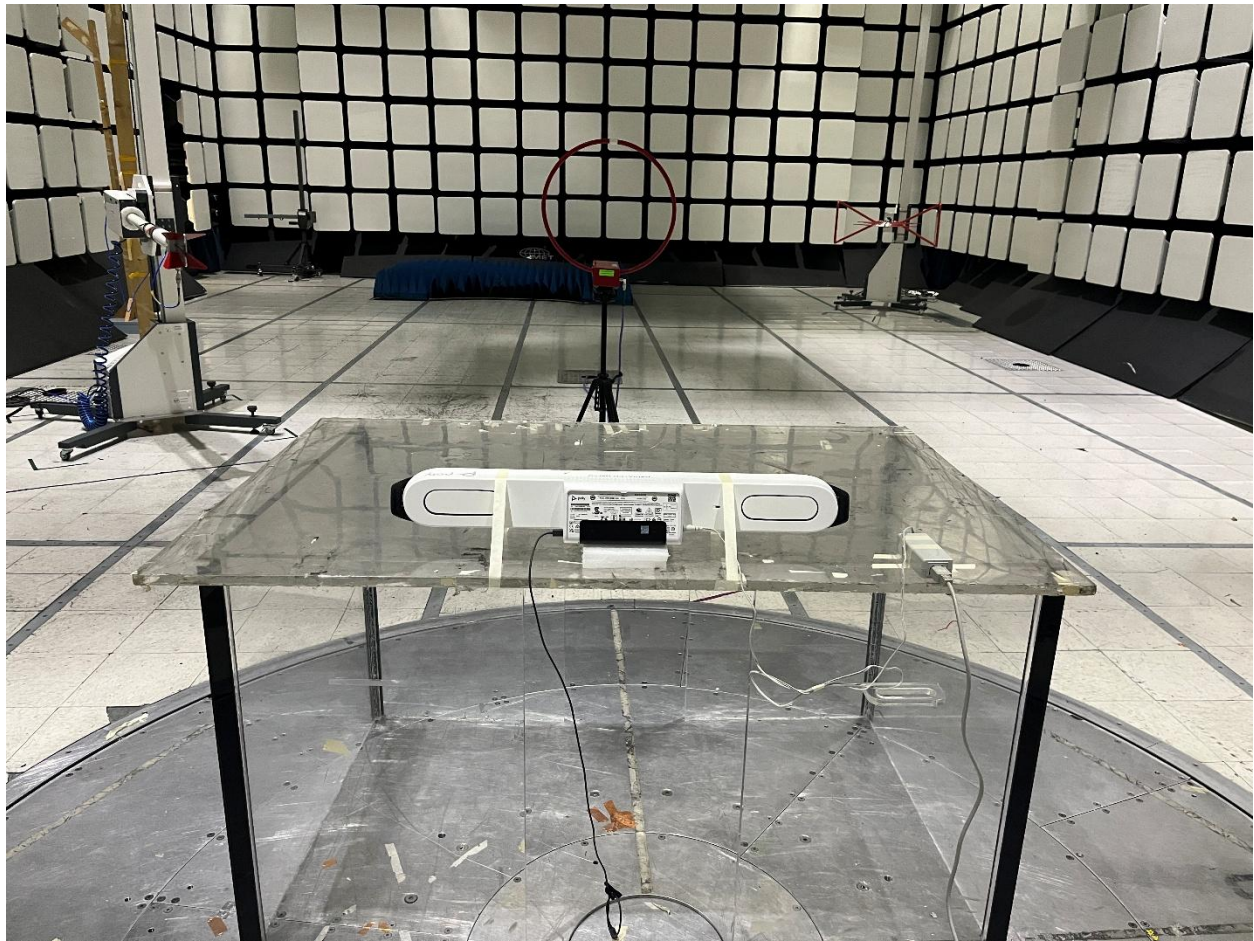
Radiated Emissions 9kHz – 30MHz (Back Side)
