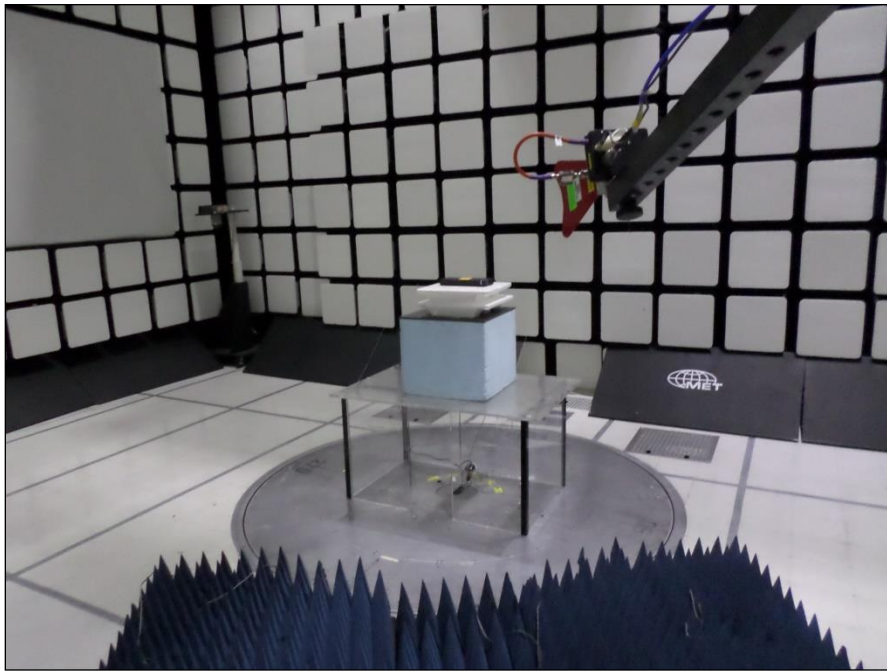
Photograph 7. Radiated Spurious Emissions, Test Setup, Above 1GHz, Antenna View
