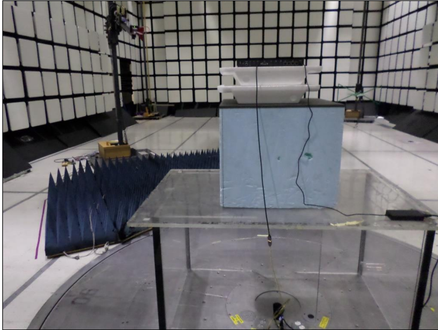
Photograph 6. Radiated Spurious Emissions, Test Setup, Above 1GHz, Rear View
