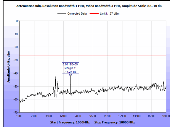
Plot 17. Radiated Emissions, 802.11ac 40, 5190 - 1-18GHz
