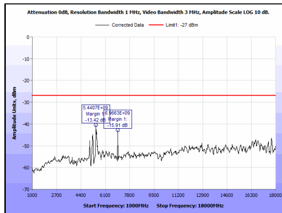
Plot 18. Radiated Emissions, 802.11ac 40, 5230, 1-18GHz
