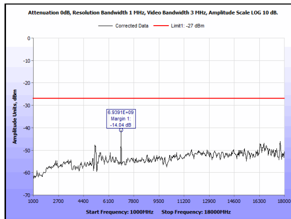
Plot 19. Radiated Emissions, 802.11ac 80, 5210, 1-18GHz
