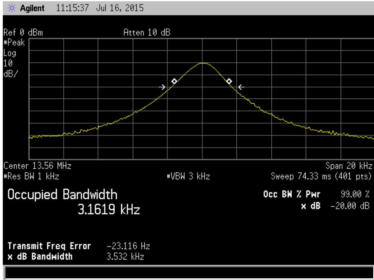
Figure 2. Occupied Channel Bandwidth of Fundamental Emission
