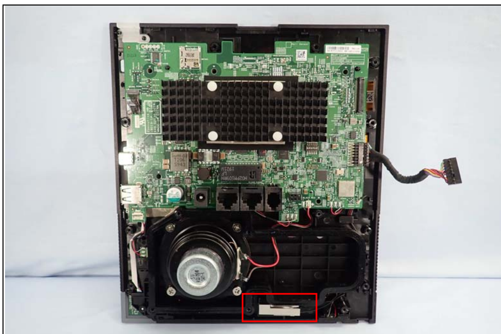
PCB antenna
