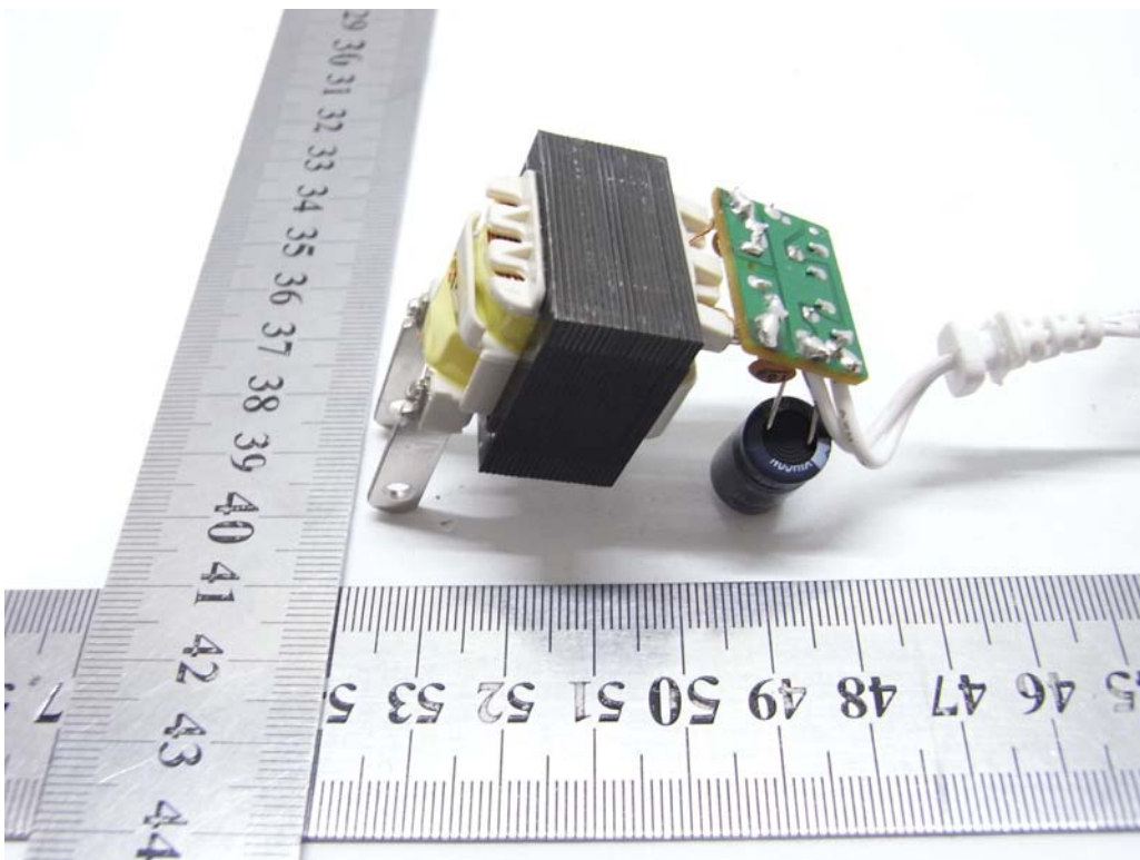
INTERNAL PHOTO OF ADAPTER
