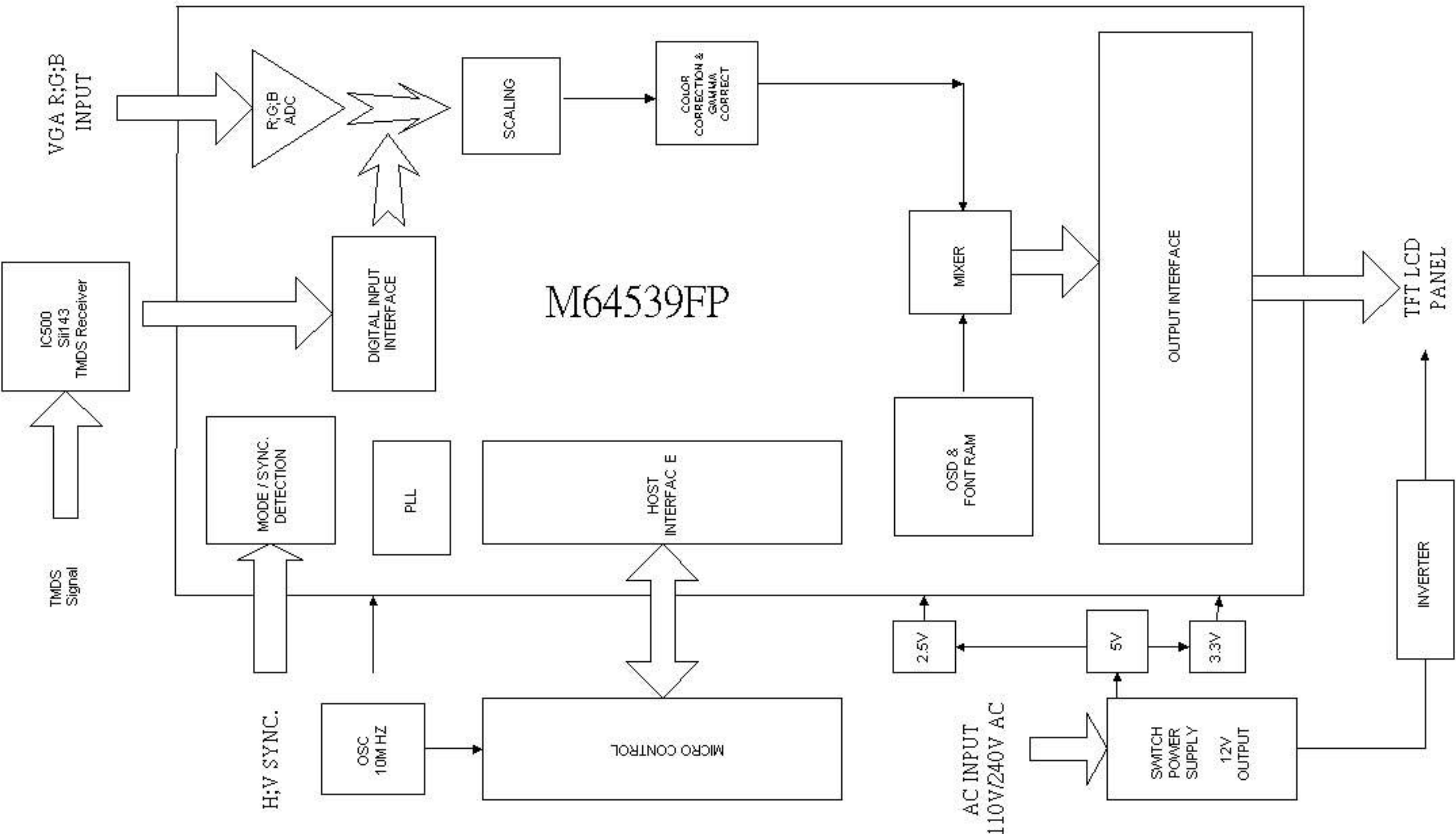
NL1502 BLOCK DIGRAM
