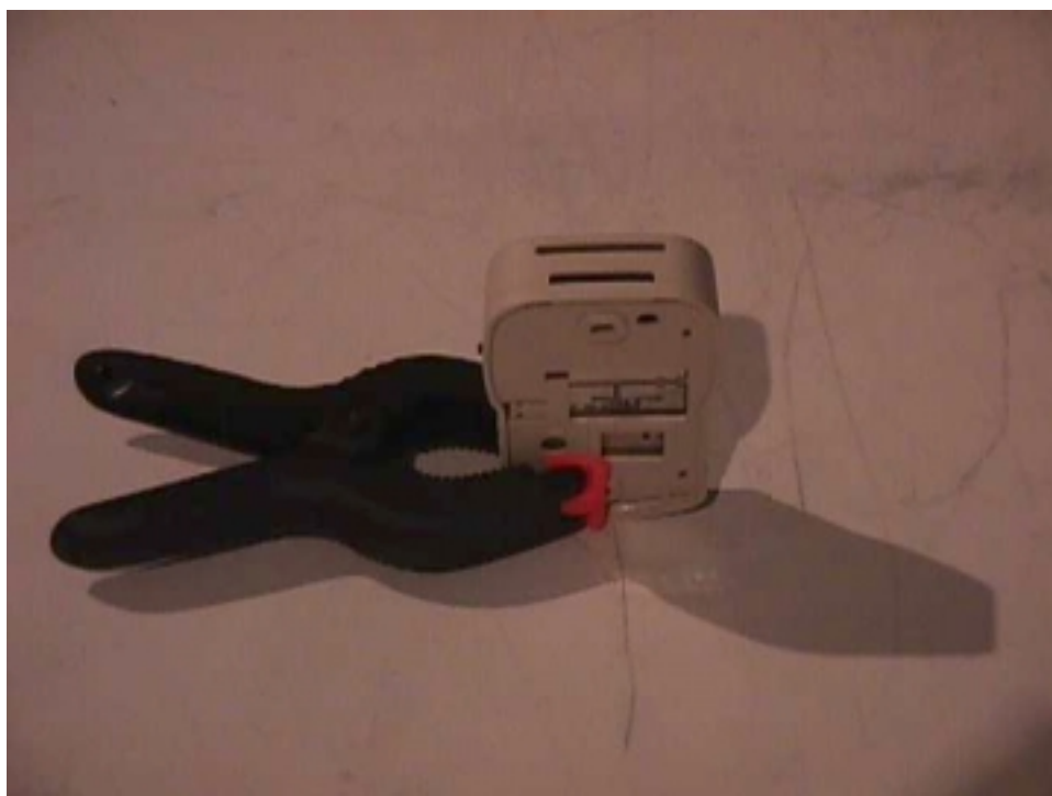
FCC RADIATED-EMISSIONS & BANDWIDTH TEST CONFIGURATION HWSO 5m SEMIANECHOIC CHAMBER LEXMARK INTERNATIONAL, LEXINGTON KY.
