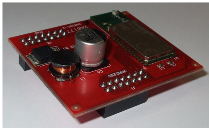
Wireless Board
