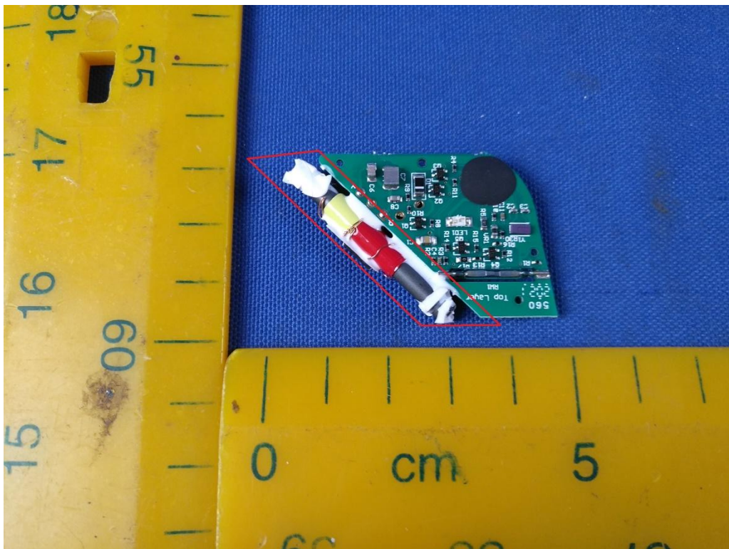
Antenna Position
