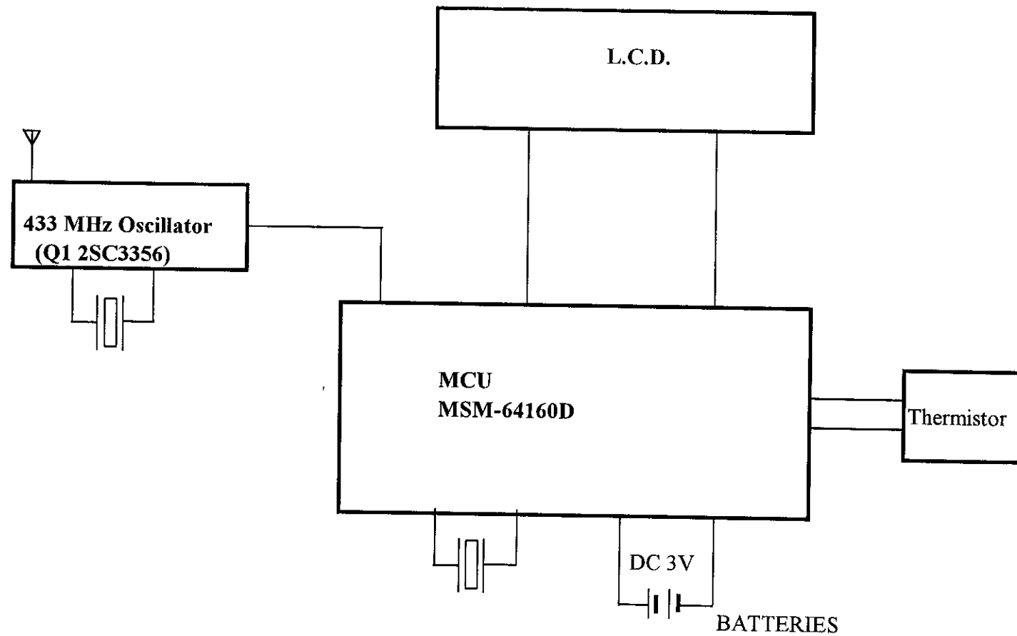
W-288R BLOCK DIAGRAM
