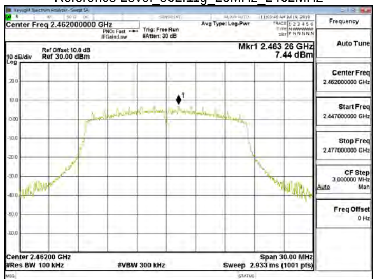
Reference Level 802.11g 20MHz 2462MHz
