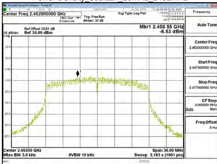
Power Density 802.11n 20MHz 2462MHz
