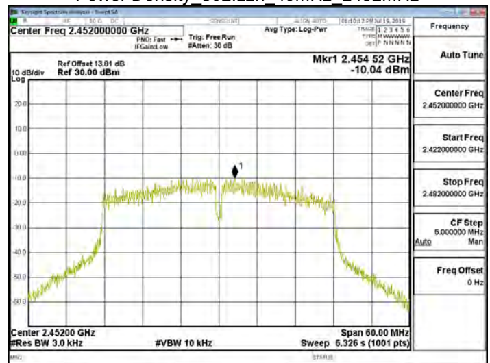
Power Density 802.11n 40MHz 2452MHz
