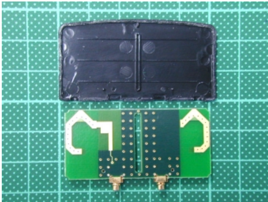
Photo 2: Antenna photo
