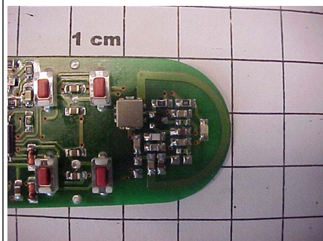
PHOTO N°1 – E.U.T. IDENTIFICATION
