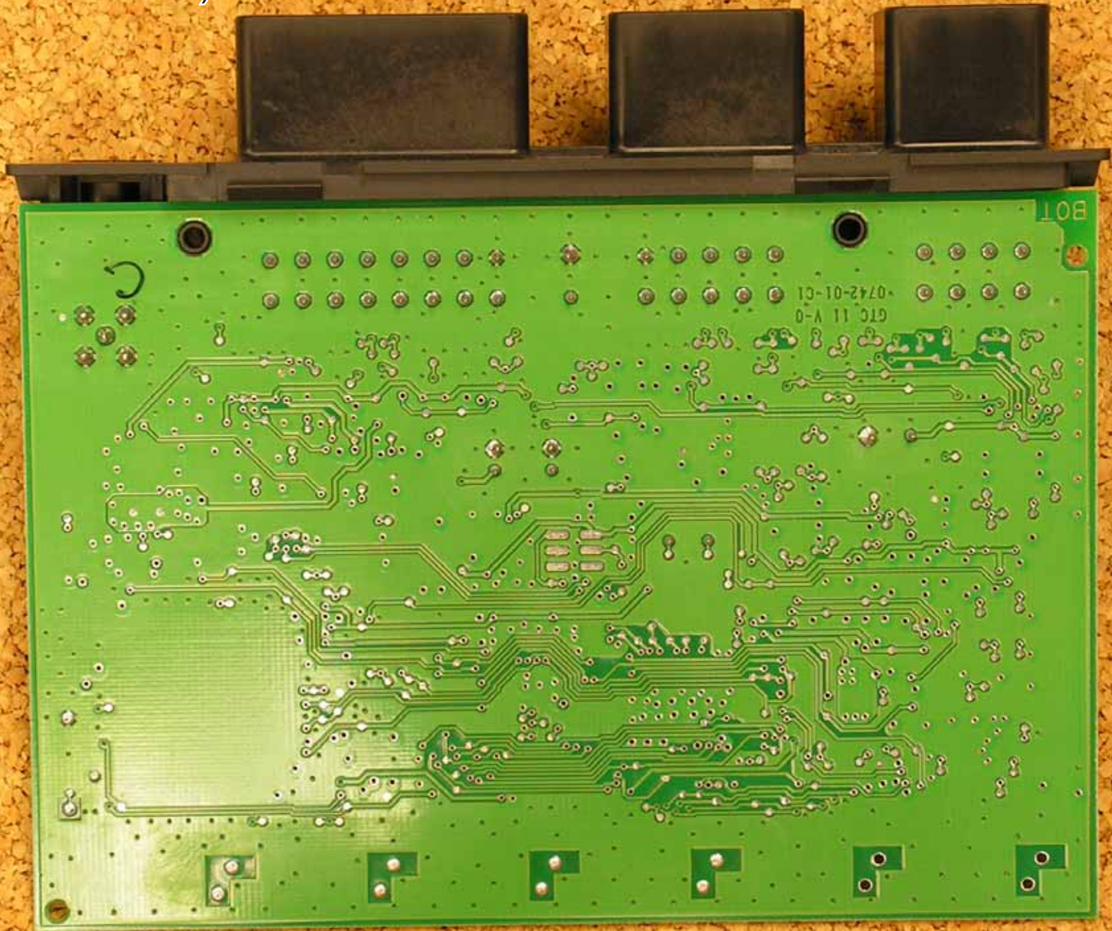
PCB (bottom)
