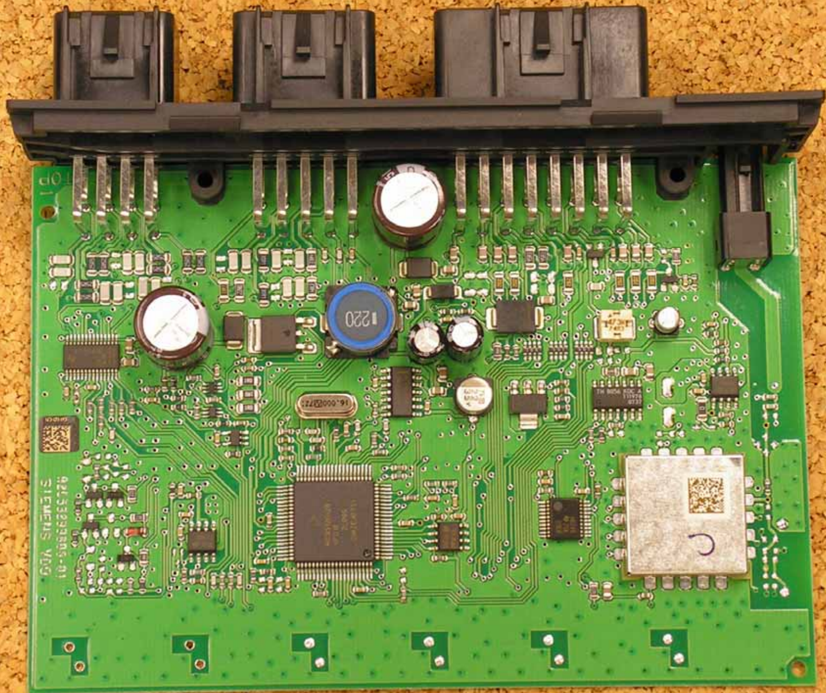
PCB (top)
