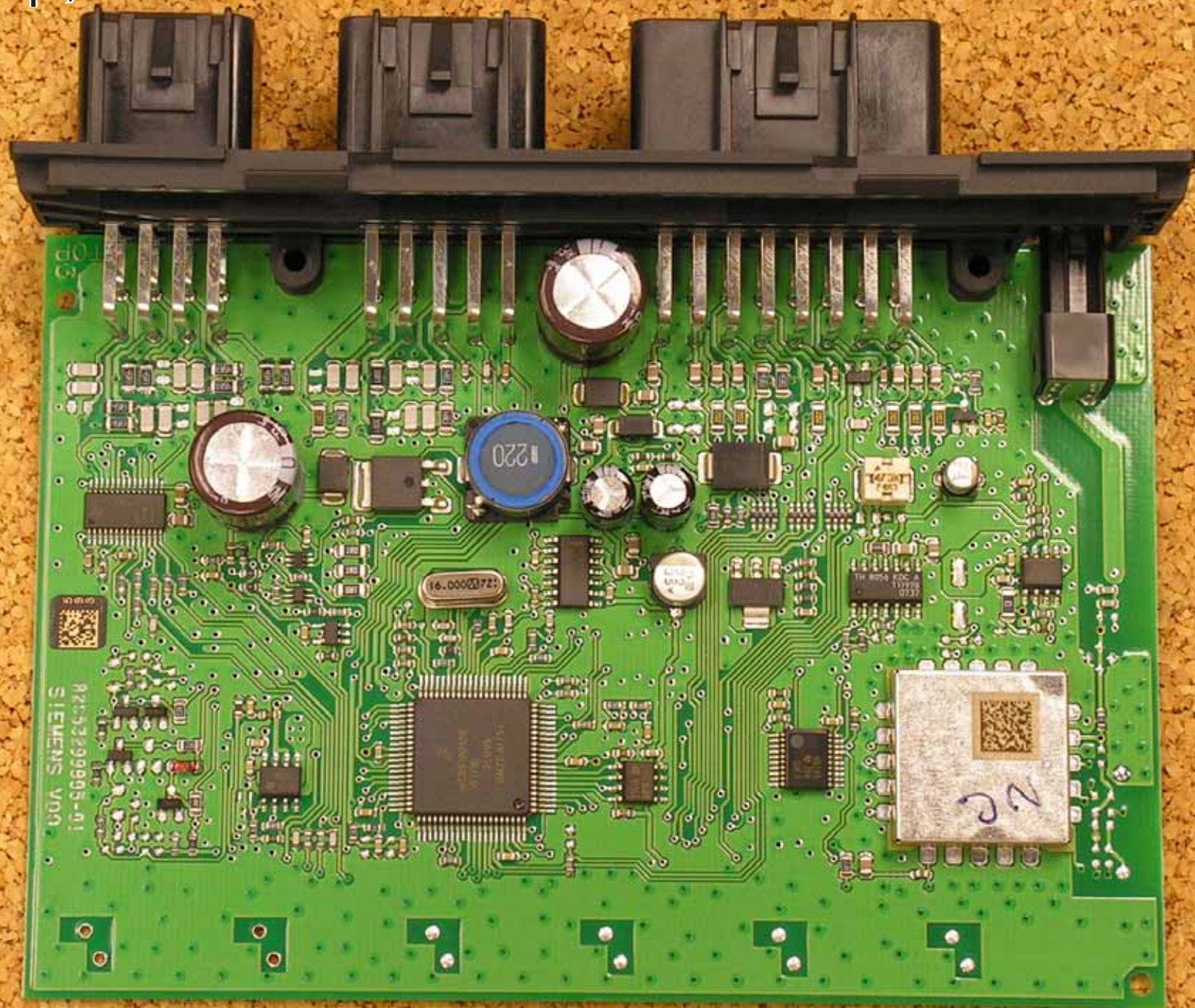
PCB (top)
