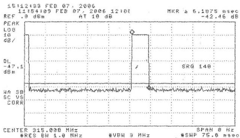
Figure 6.1(c). Transmissions modulation characteristics (LF Actuation): (top) complete transmission, (center) expanded bit, (bottom) expanded period.
