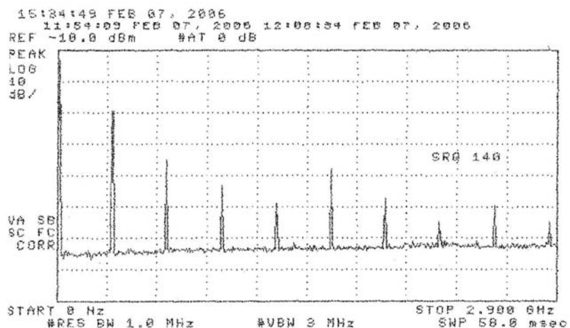
Figure 6.2. Emission spectrum of the DUT (pulsed emission). The amplitudes are only indicative (not calibrated). (top) RKE, (bottom) RS
