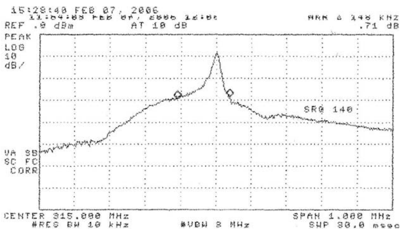
Figure 6.3. Measured bandwidth of the DUT (pulsed emission). (top) RKE, (bottom) RS
