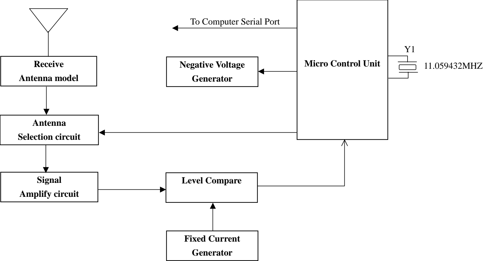
PEN20 RS232 Circuit Function Block Diagram
