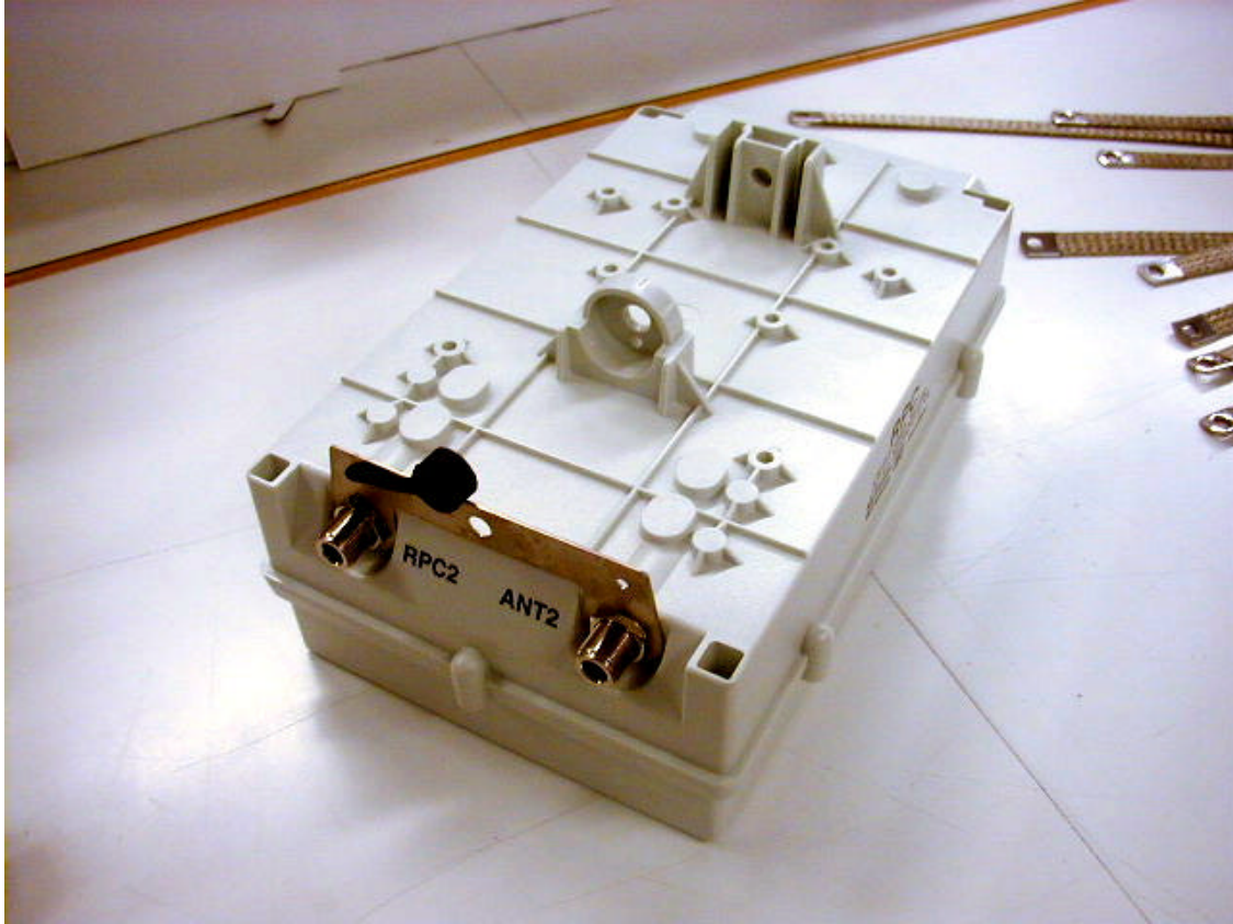
PRC-unit, top side
