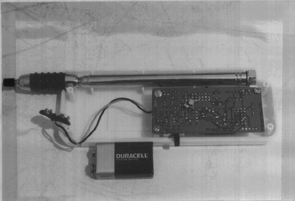
Back Cover Removed showing location of PWB and Antenna
