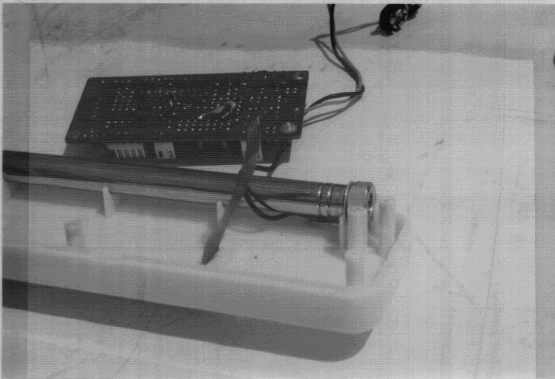
Antenna Mounting and Ribbon Cable to Keypad Antenna is a YH860501 part manufactured by Ying Hao Metal Industries LTD.
