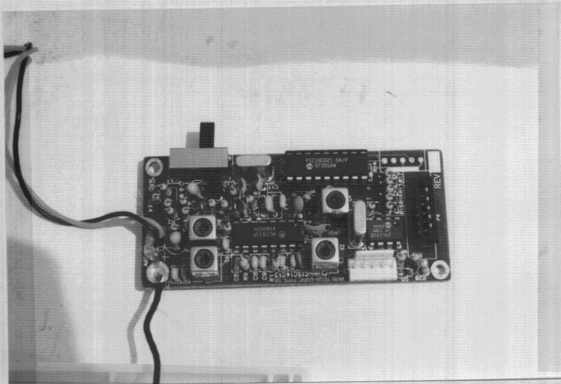
Transmitter PWB - Component Side
