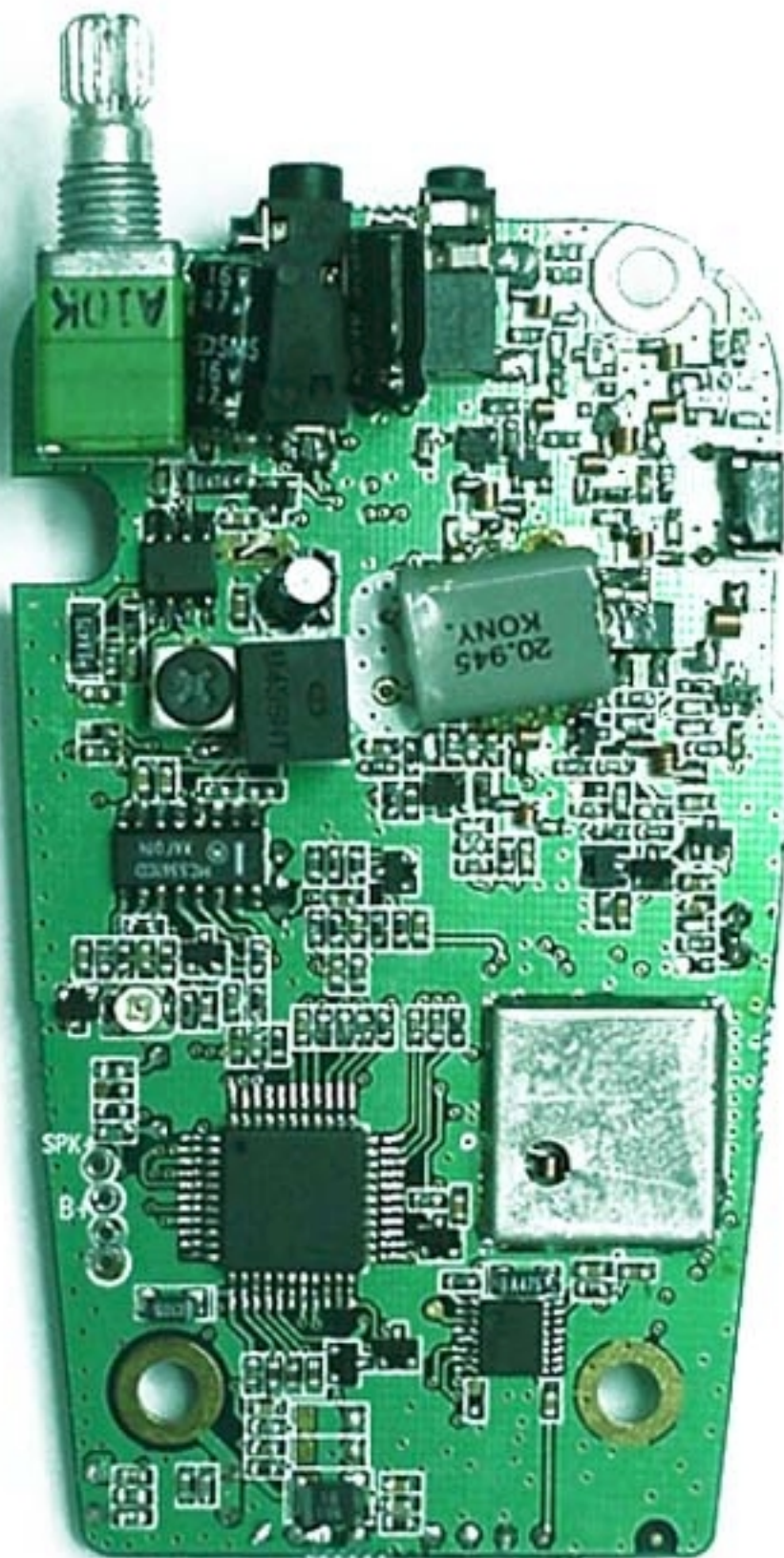
PCB – Bottom
