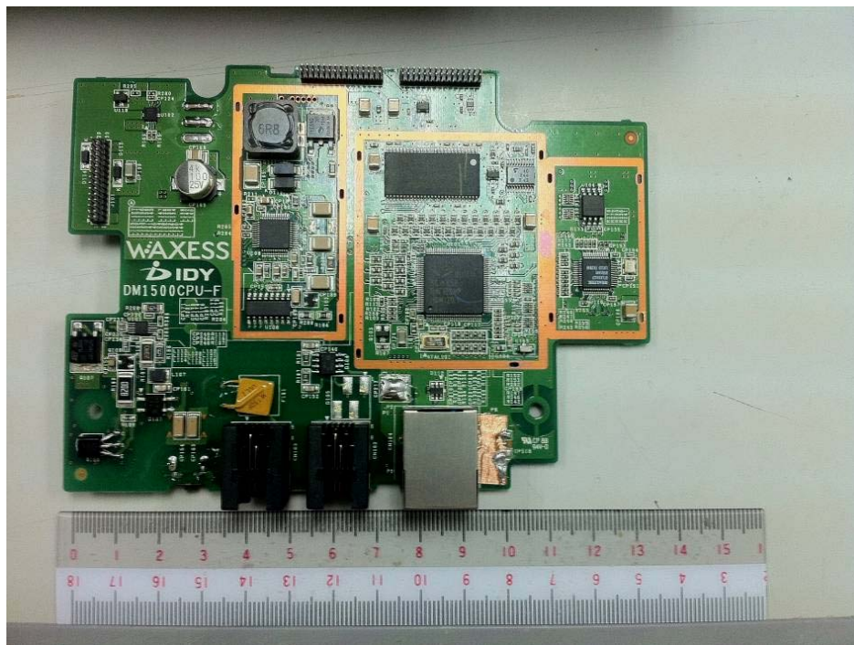
EUT – DM1500-CPU-F Board Top Shielding Off View
