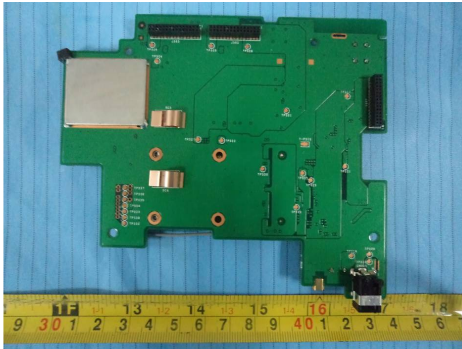
EUT – DM1500-SUB-E Board Bottom Shielding off View
