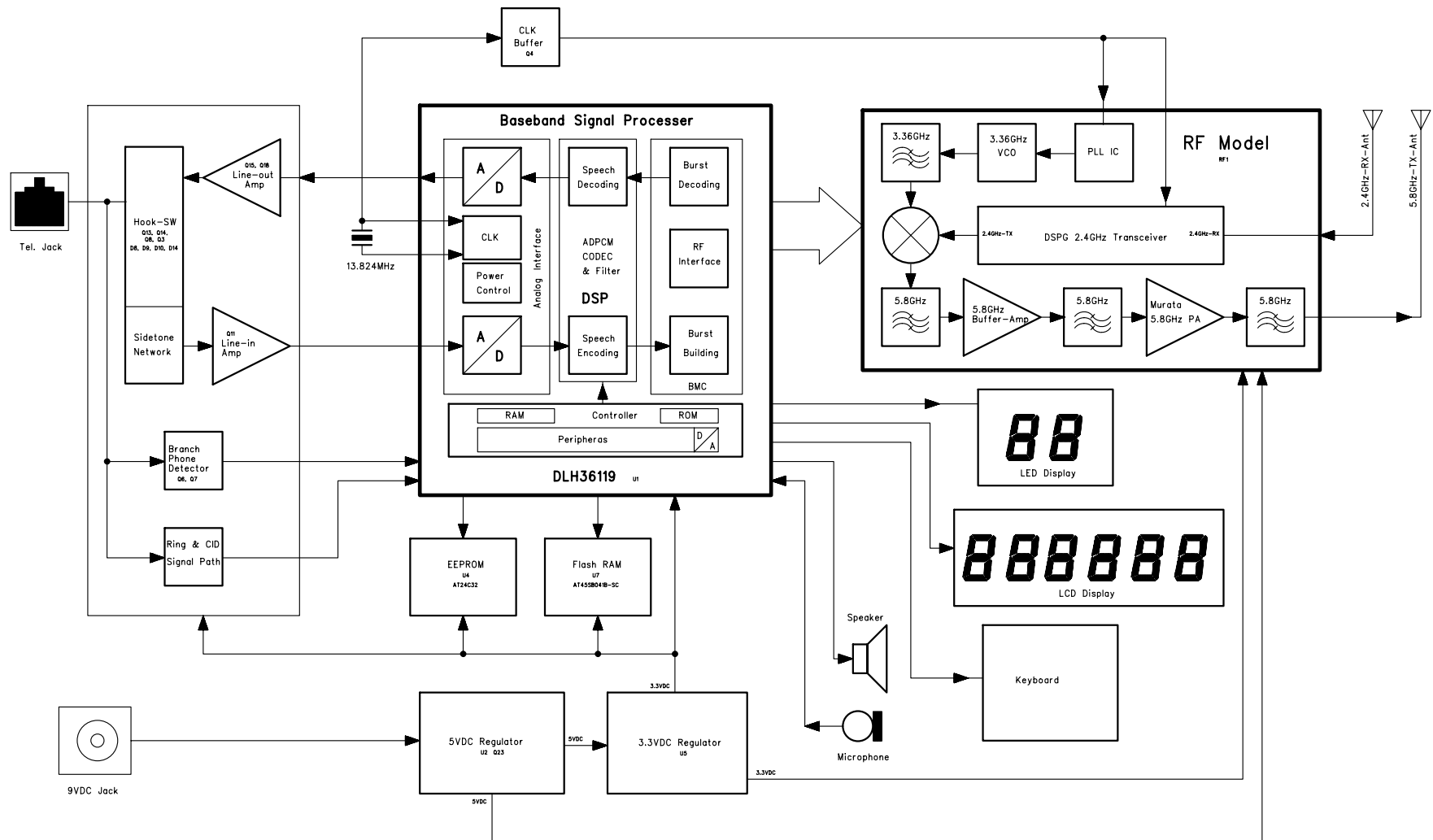
NWB35818 Base Unit Block Diagram
