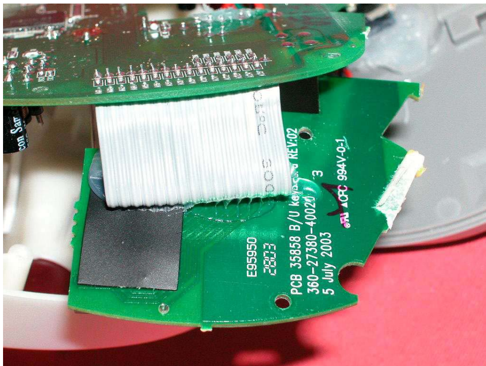
Base DAM keypad PCB rear side (View 1)
