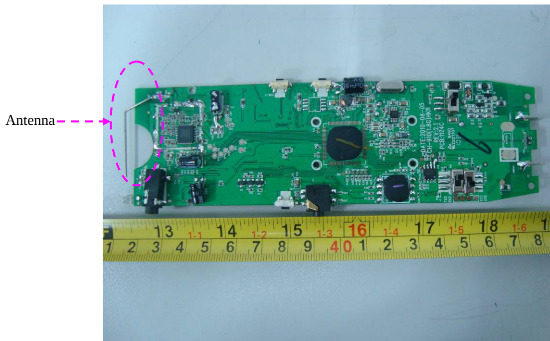
EUT – Main Board Top Shielding off View
