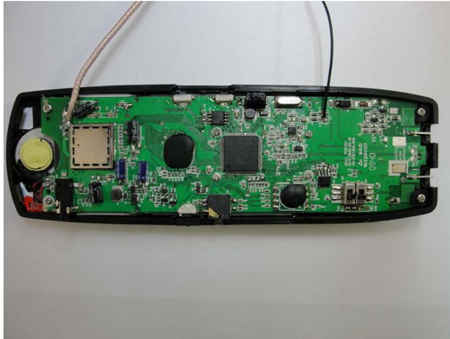
Figure 1: EUT Internal View (back of LCD)
