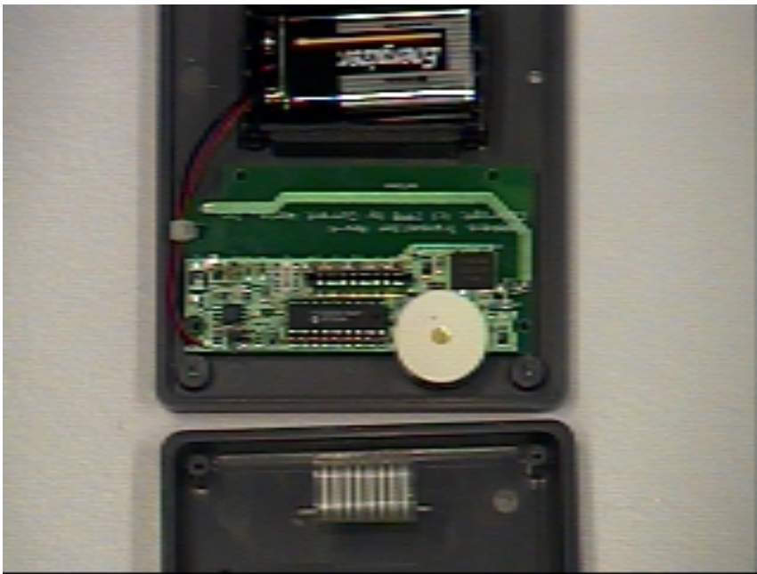
Component side of PCB with ribbon cable showing
