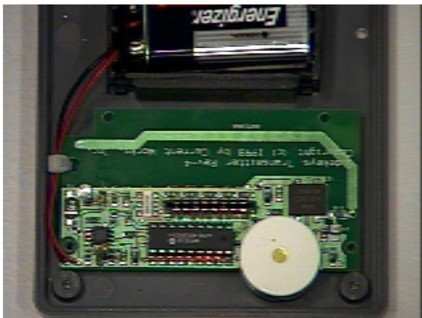
Component Side of PCB
