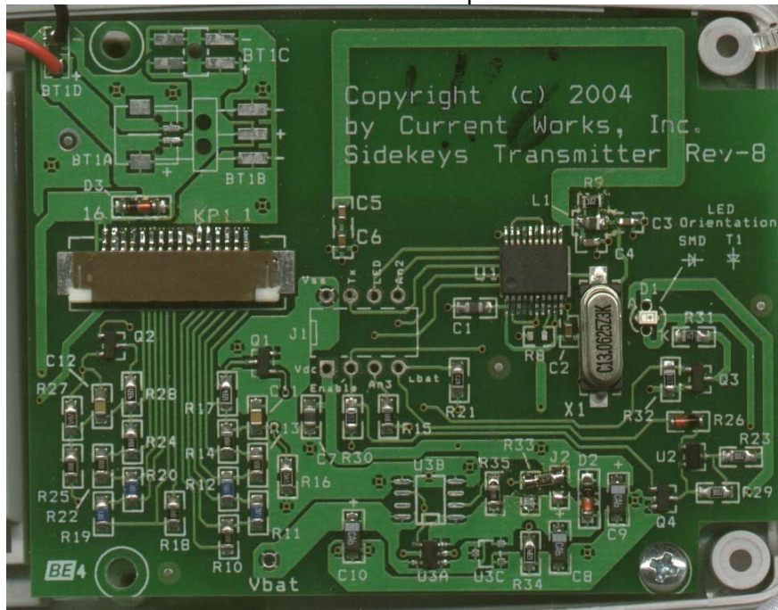
Processor Board – Component Side
