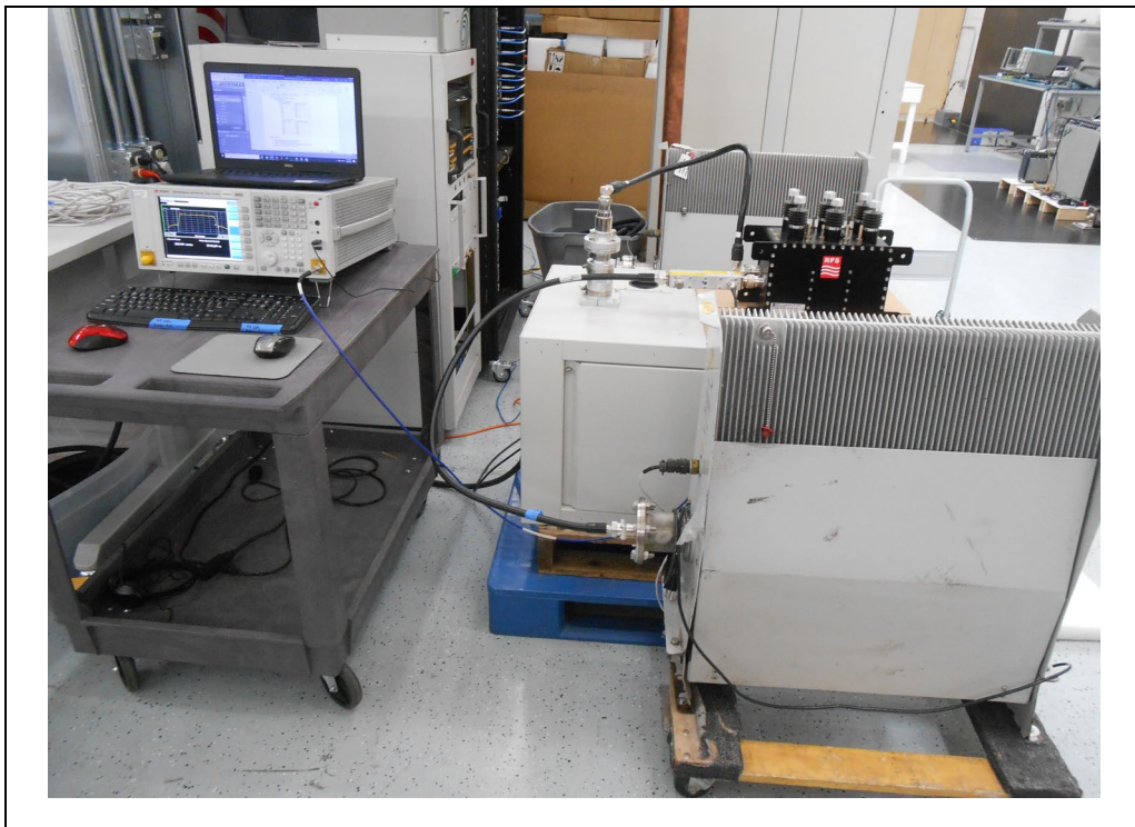
RF Conducted #2
