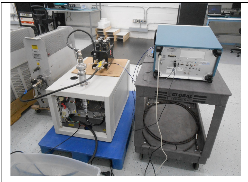
RF Conducted #2
