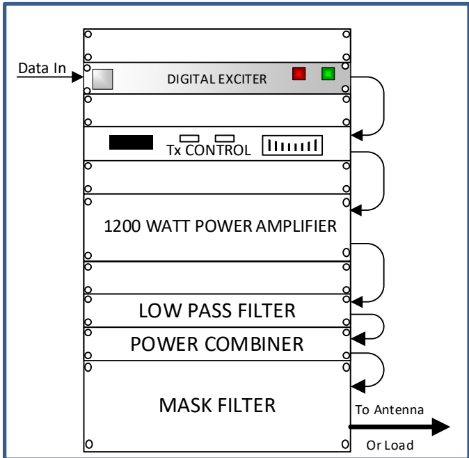
Figure 4-1 TX System Operating Signal Flow Chart
