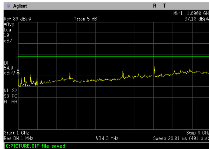
Figure 5-16 Vertical Radiated Emissions Plot above 1 GHz
