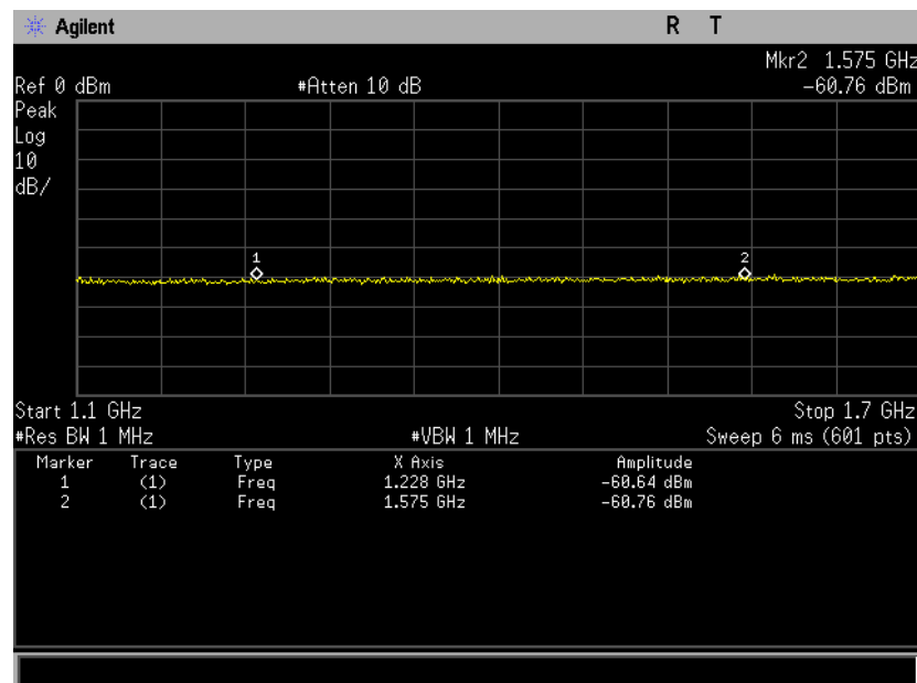
Figure 5-10 Radiation into Radio Navigation Satellite Services (GNSS/GPS)
